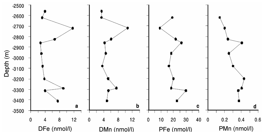
Figure 3. Vertical distribution of (a) dissolved iron, DFe, (b) dissolved manganese, DMn, (c) particulate iron, PFe and (d) particulate manganese, PMn in water column at CTD-16 (05°53.9'N, 61°06.3'E).
