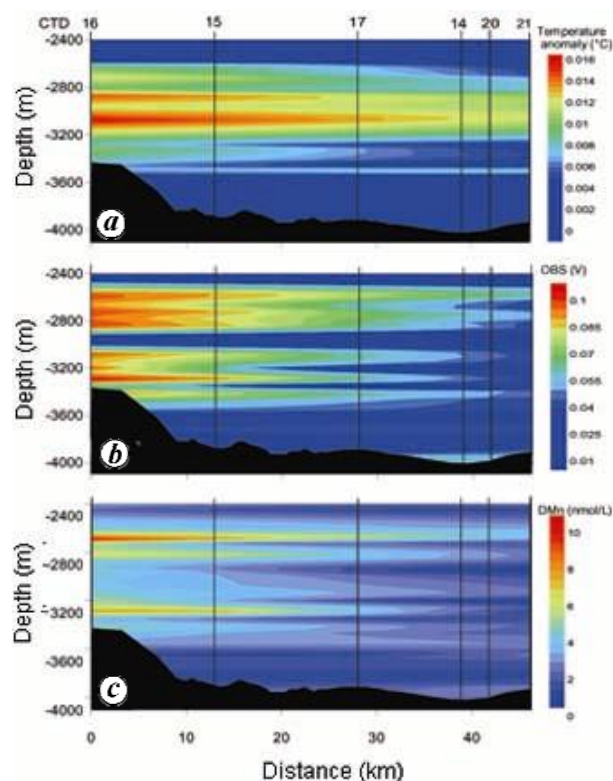
Figure 2. Two-dimensional transects of water column: (a) Potential temperature anomaly ( ^{\circ}\text{C} ); (b) optical backscatter signals (V) and (c) dissolved manganese (nmol/l) along the axial rift valley. The intense temperature anomaly was found as a broad band between 2850 and 3150 m, unlike two separate layers of DMn and optical backscatter signals appear between 2500–2900 m and 3100–3400 m. As density gradient limits the depth distribution of non-buoyant plumes, the DMn, plume particulates remain in suspension and slowly disperse horizontally over a distance 16 . The hydrothermal heat on the other hand, dissipates fast in all directions. Hence receiving heat from both the plumes, the intermediate (2850–3150 m) water mass would be expected to have maximum temperature anomaly.
