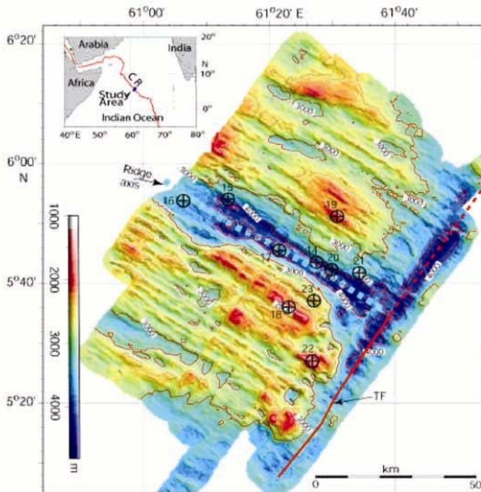
Figure 1. Sea-floor topography generated from swath bathymetry of survey area along with CTD hydrocast locations on Carlsberg Ridge. Spreading centre and transform fault (TF) are marked with contour interval of 500 m.
