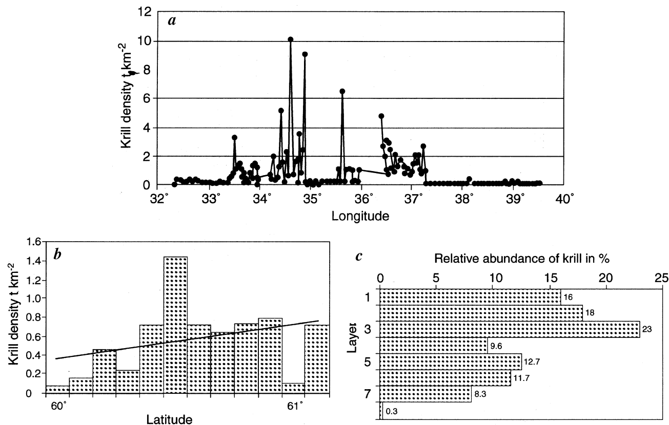
Figure 3. a , Krill biomass density distribution along 61°S lat. b , Trends in krill density distribution in sub-area between lat 60°00' and 61°15' S lat. c , Relative vertical distribution of krill biomass in sub-area between lat 60°00' and 61°15' S (layer thickness = 15 m).
