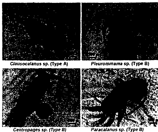
Fig. 4—Tumors observed in different copepod genera.
