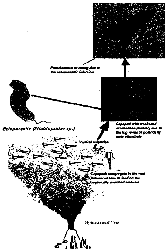
Fig. 7—Schematic representation of the possible relationship between hydrothermal plume and Tumor like anomalies in planktonic copepods
