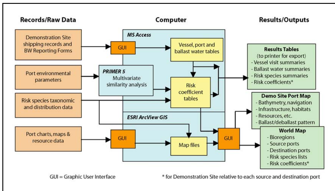
Figure 3. Schematic of the GloBallast BWRA system
