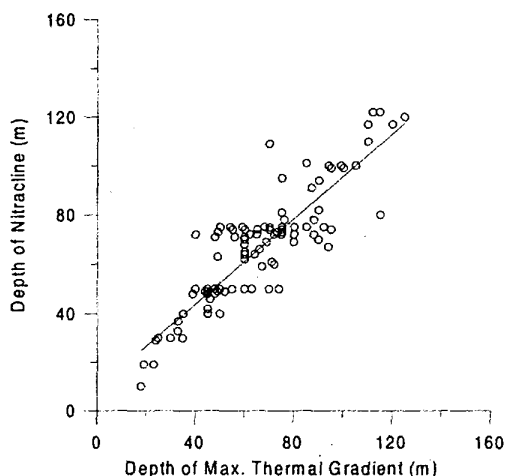
Fig. 4. Linear regression between the depth of the nitracline and the depth of thermocline ( n=127 ) in the southwest and the intermonsoon seasons in the Arabian Sea.
