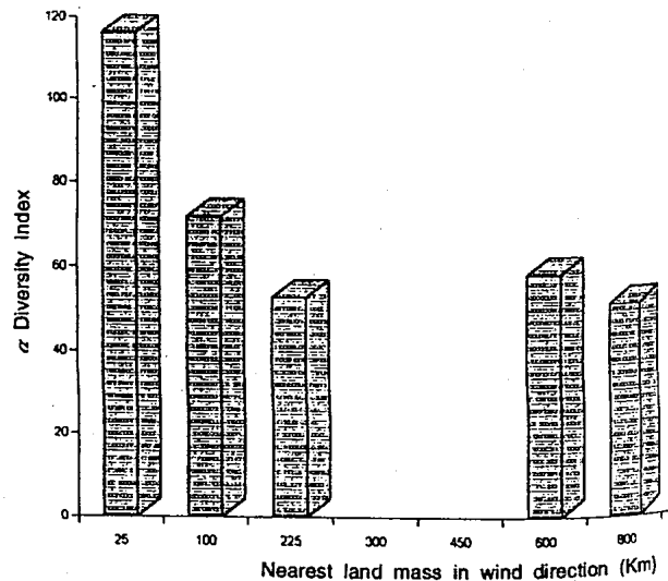
Figure 5. Column chart showing \alpha diversity index of air borne insects trapped in relation to the distance of the nearest land mass in wind direction.
