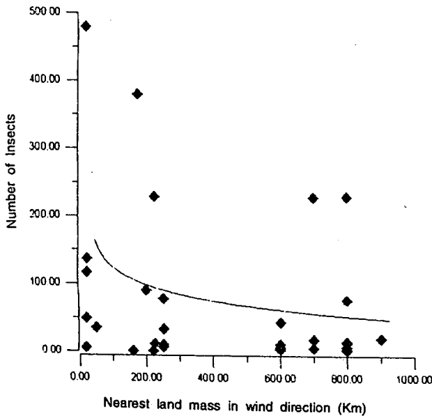
Figure 4. Curve showing the relation between the number of insects trapped in northern Arabian sea and the distance of the nearest landmass along the wind direction. The best fit for the curve was \log Y = B \log (X) + A .
