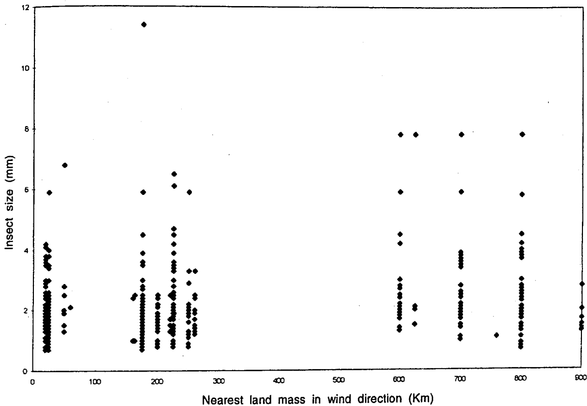
Figure 7. Scatter plot showing the relation of insect size and the distance of the nearest land mass in wind direction.
