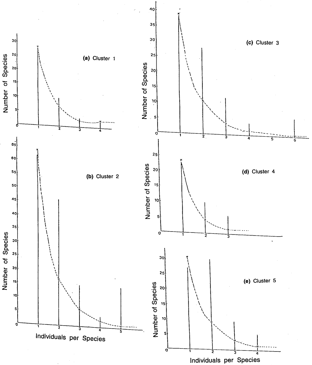
Figure 6. Frequency distribution of the insects in the five clusters. Vertical lines show the number of individuals per species. Crosses joined by broken lines show the log series.
