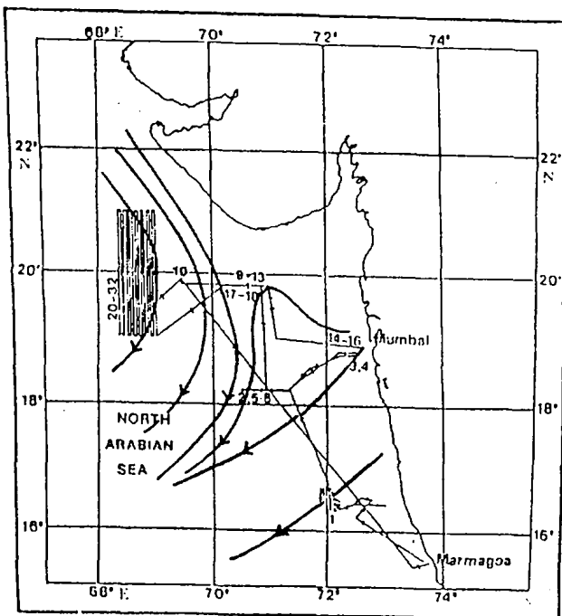
Figure 1. Track of cruise No. 111, ORV SAGAR KANYA in the northern Arabian sea during March–April 1996. Numbers along the track indicate sampling stations for air borne insects. Superimposed on the track is the generalized wind flow pattern during the period.
