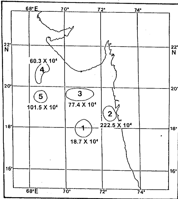
Figure 3. Aerial density (per km 3 ) of insects in different clusters of the study area in Arabian sea.
