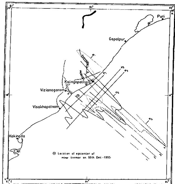
Figure 2. Magnetic anomalies along 3 parallel profiles.
