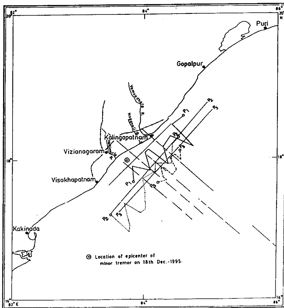
Figure 4. Magnetic basement inferred from model studies.
