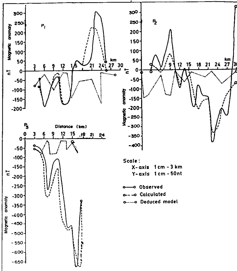
Figure 3. Two-dimensional models of 3 anomalies.
