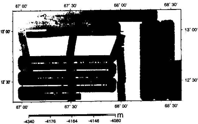
Figure 2. Grey shaded depth contour map showing the meandering channels.
