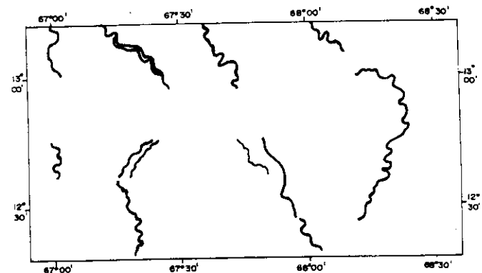
Figure 3. Traced paths of the deciphered channels.
