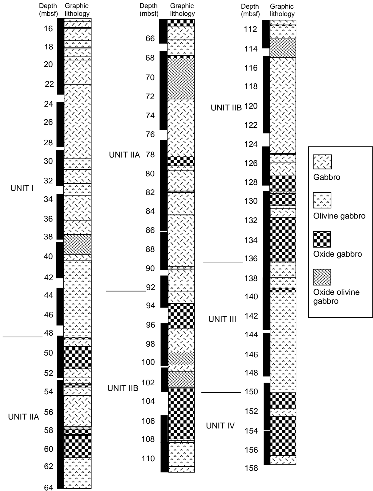
Figure F3. Summary of visually defined lithologic intervals and syntheses units of Hole 1105A. Only the main lithologic rock types are illustrated.
