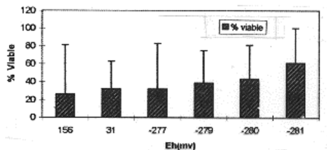
Figure 1. Bacterial viability at different Eh ( n = 10 for oxidizing and 20 for reducing conditions).
