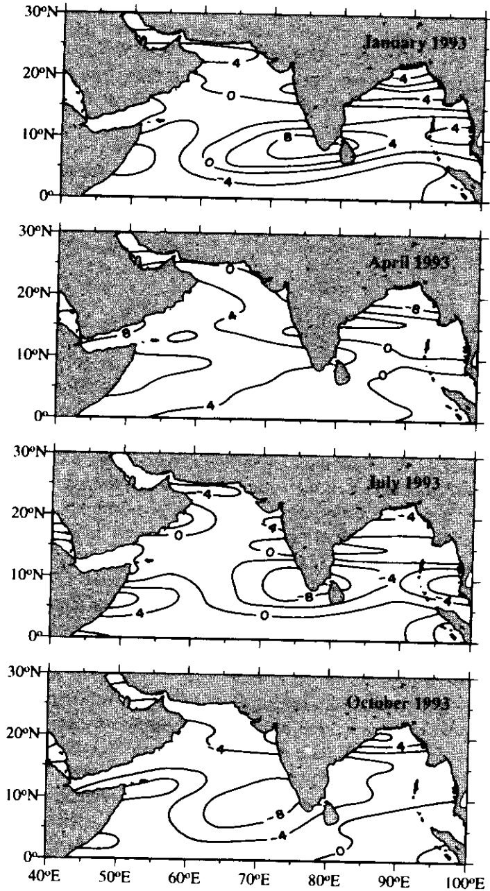
Figure 2. Sea level deviation for 1993 from TOPEX/POSEIDON. The mean level was defined over 1993–1995. The deviations, computed along the TOPEX/POSEIDON tracks, were averaged in 4^\circ \times 1^\circ (longitude by latitude) cells to construct regular monthly grids of sea level change. Taken from Shankar & Shetye (1997).
