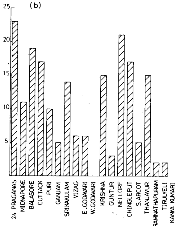
Fig. 1. Preferred strips along the Indian coasts which are more vulnerable to tropical cyclones
