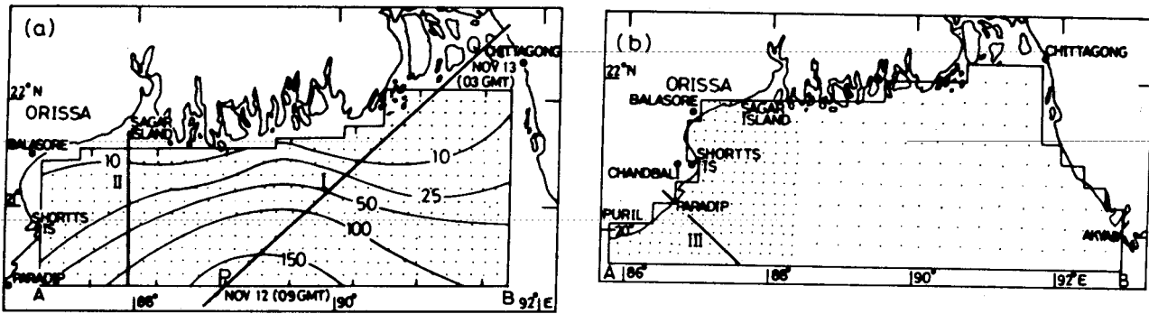
Fig. 3. Grid scheme for three different types of tracks
