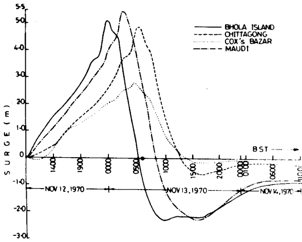
Fig. 20. Model computed peak-surge at Chittagong
