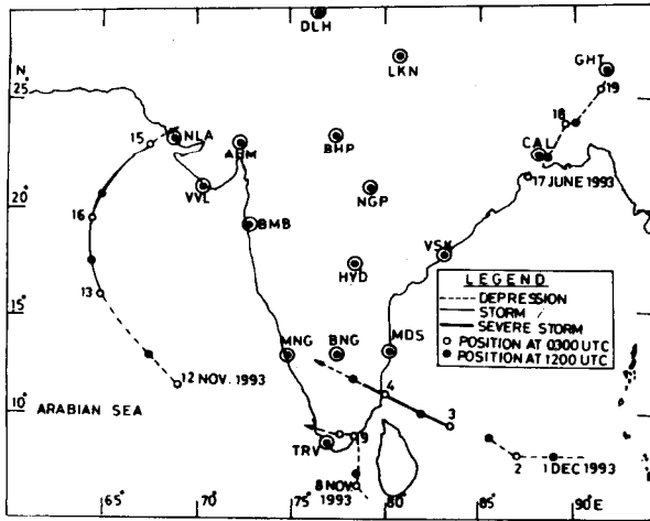
Fig. 17. Karaikal cyclone (December 1993)
