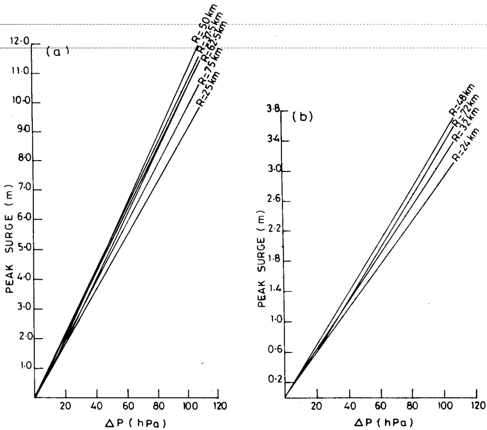
Fig. 5. Same as Fig. 4 but for the northern part and remaining part of the coast
