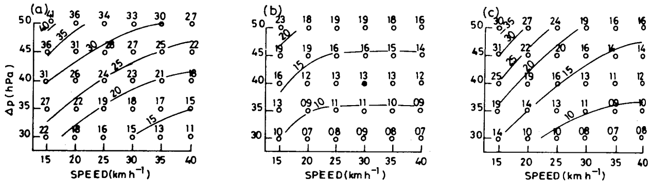
Fig. 4. Nomograms for the storm surges as a function of the storm intensity and speed of movement of cyclone
