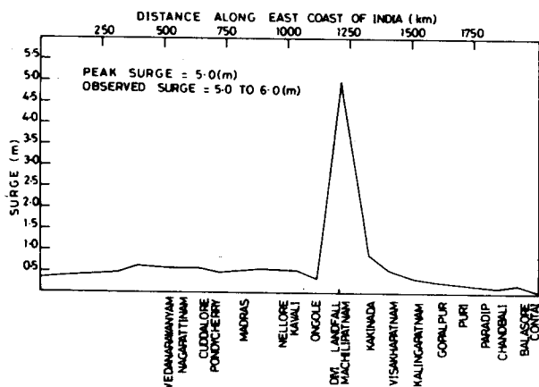
Fig. 10. Model computed peak surge values associated with Andhra cyclone closest to Divi Island
