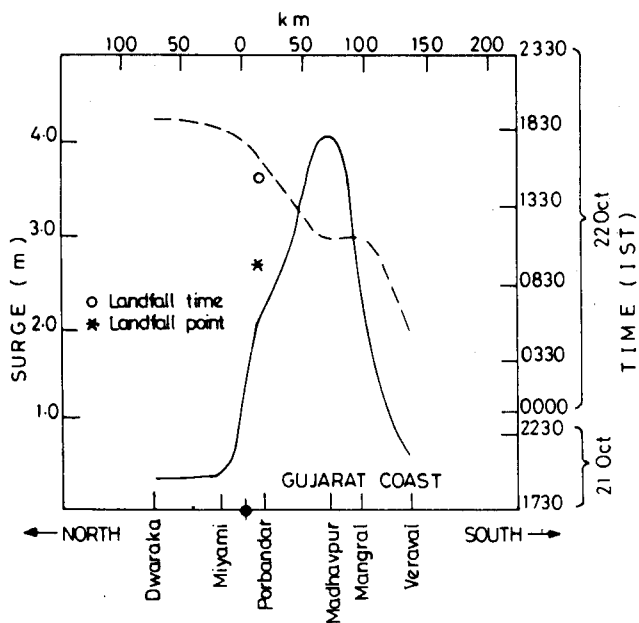
Fig. 26. Distribution of the predicted maximum sea surface elevations, observed surge and the time of occurrence along the Gujarat coast.
