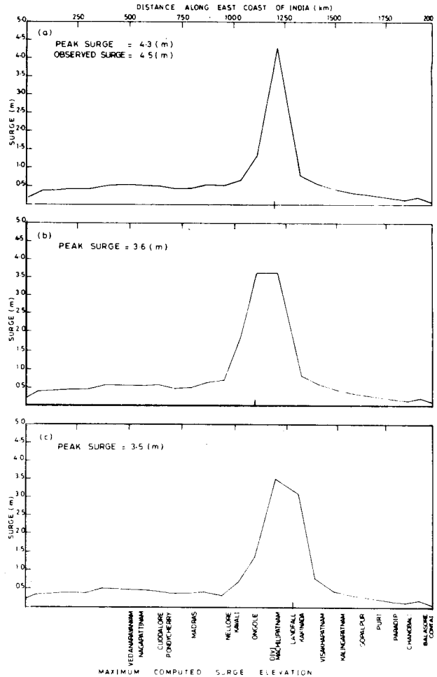
Figs. 14(a-c). Model-computed peak surge envelop (a) along the east coast of India, (b) when the landfall of cyclone is 100 km to the north and (c) when the landfall of the cyclone is 100 km to the south
