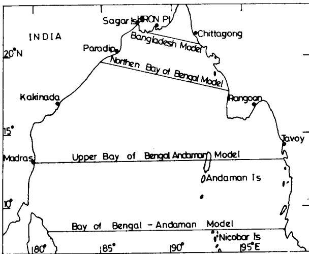
Fig. 6. Regular grids
