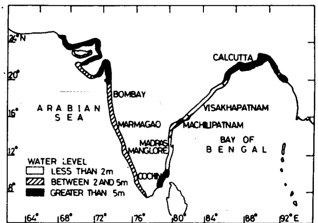
Fig. 2. Classification of the Indian coast into three types of vulnerability to storm surges (After Rao 1968)
