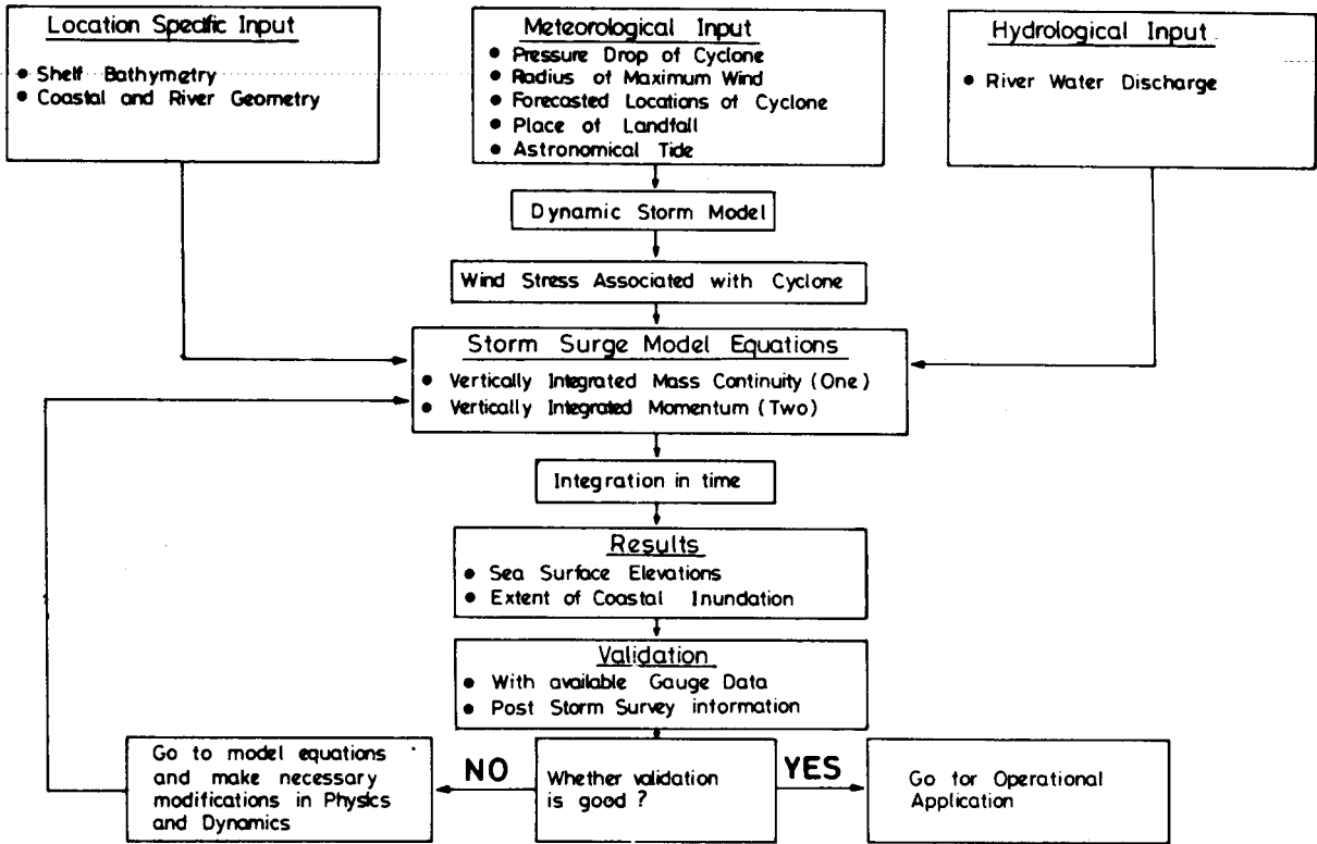
Fig. 8. A model for real time storm surge prediction system
