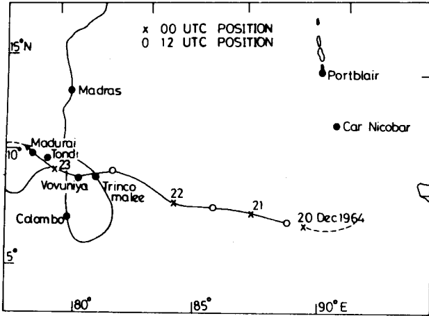
Fig. 23. Sri Lanka : Rameswaram cyclone (December 1964)
