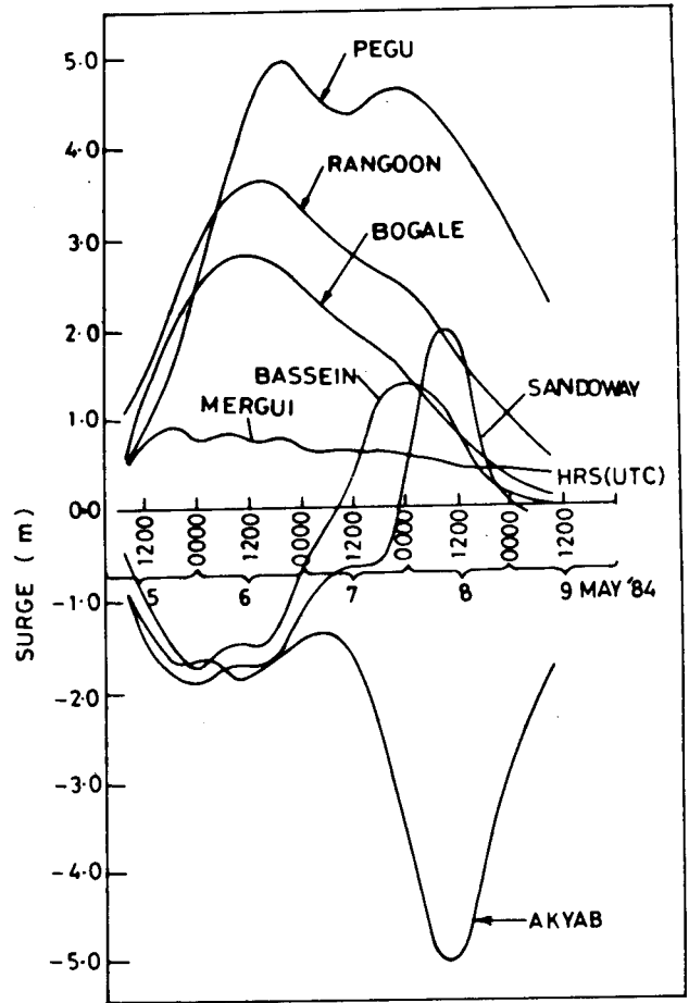
Fig. 22. Time variation of the sea surface elevation at selected stations
