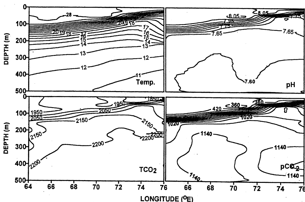
Figure 4. Distribution of temperature (°C), pH, TCO 2 (µM) and pCO 2 (µatm) along an east-west section around 10–11° N.
