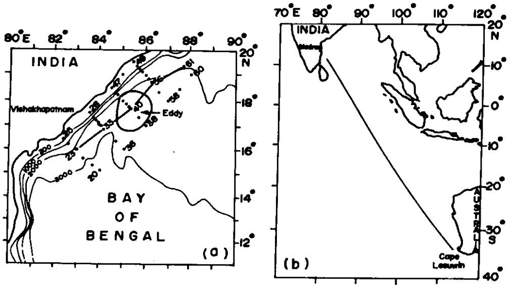
Fig. 1 - Location of sections considered for this study, a) across a cold core eddy in the western Bay of Bengal, b) Cape Leeuwin (Australia) to Madras
