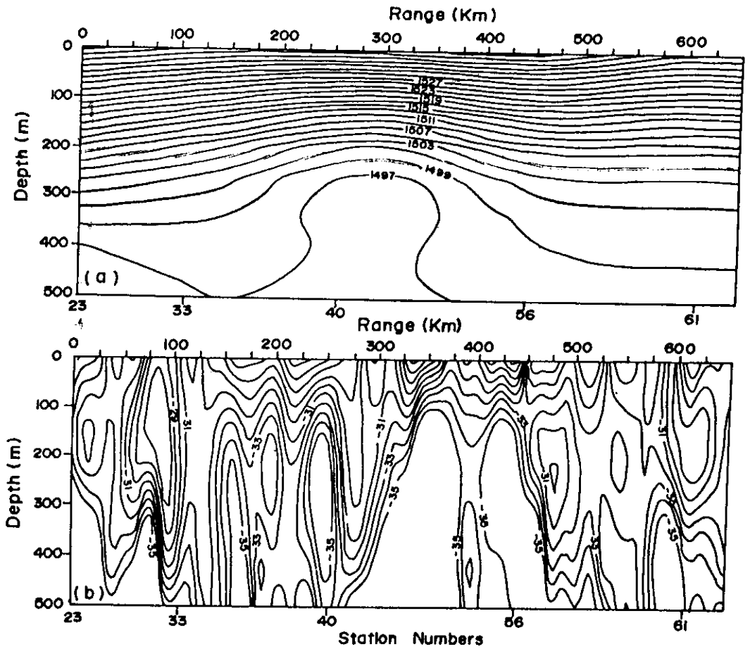
Fig. 2 - a) Vertical section of sound speed across the subsurface cold core eddy in the western Bay of Bengal, b) contours of acoustic intensity levels computed using IFD program
