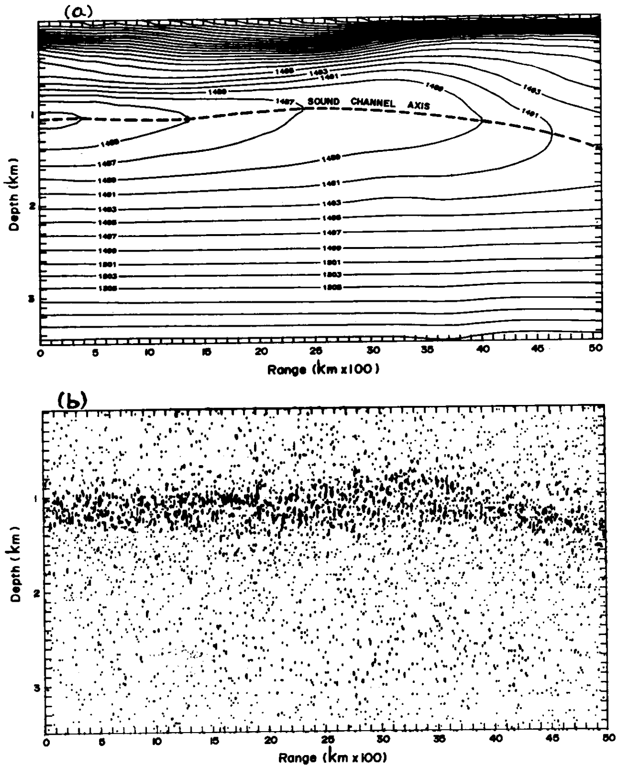
Fig 3 – a) Vertical Structure of sound speed from Cape Leeuwin (Australia) to Madras along the Geodesic path, b) contours of acoustic intensity level in the SOFAR propagation
