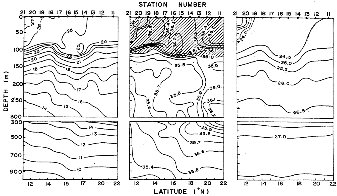
Figure 4. Vertical section of temperature (left) salinity (middle) and sigma-t (right) along 64°E during winter monsoon. Salinity >36 PSU is hatched to demarcate the Arabian Sea High Salinity Water mass.
