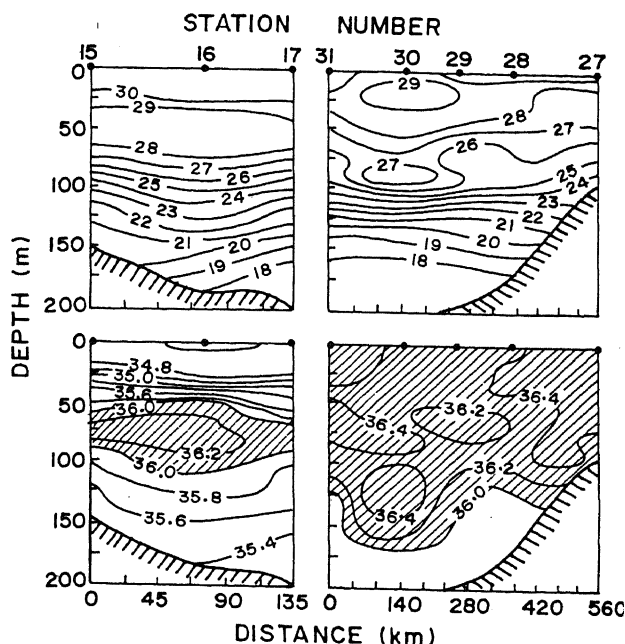
Figure 6. Vertical section of temperature (top) and salinity (bottom) along the shelf during inter-monsoon. Salinity >36 PSU is hatched to demarcate the Arabian Sea High Salinity Water mass.
