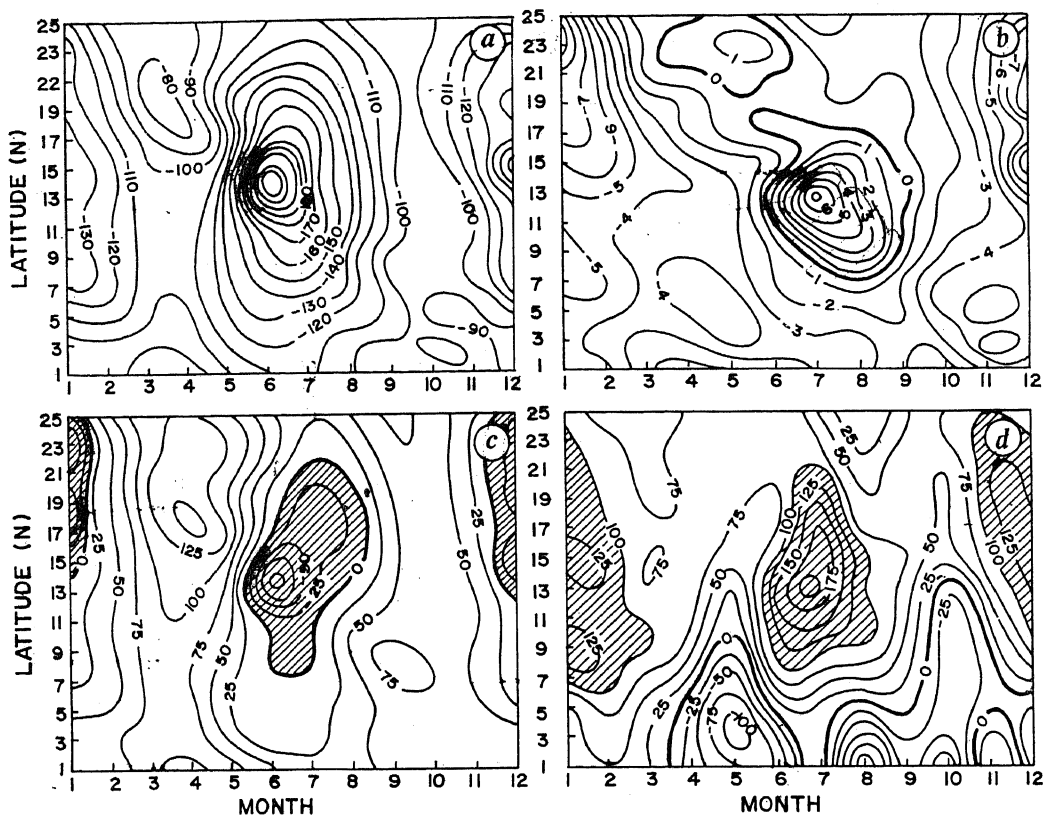
Figure 10 a-d . Time-latitude section of (a) Latent heat flux ( Q_L , \text{Wm}^{-2} ), (b) Sensible heat flux ( Q_s , \text{Wm}^{-2} ), (c) Net heat flux ( \text{Wm}^{-2} ), and (d) evaporation-precipitation (E-P, mm/month) along 64^\circ\text{E} . The hatched region in (c) represents a net heat loss while that at (d) shows where evaporation exceeds precipitation by more than 100 mm/
