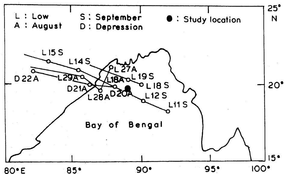
Figure 1. Area of study with trajectories of depressions.
