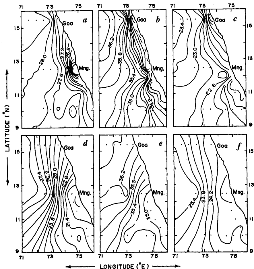
Figure 4 a-f. Horizontal distribution of temperature (a), salinity (b), and density (c) at the surface and at 50 m (d, e, f) respectively. Note the change in the contour interval of temperature at 50 m.
