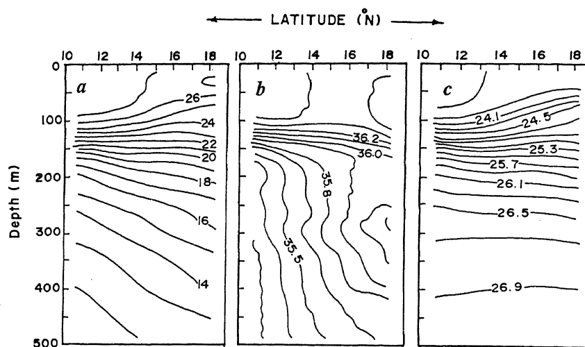
Figure 6. Vertical distribution of temperature (a), salinity (b), and density (c) along 64° E.
