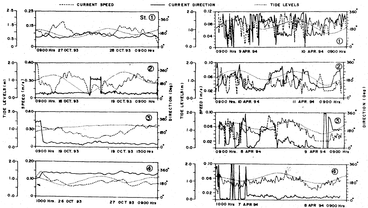
Fig. 2—Current characteristics in October and April
