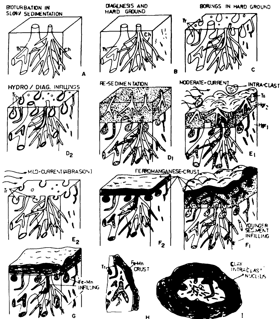
Fig. 7. Schematic diagrams depicting sequence of events in formation of pelagic hardgrounds and associated intraclast lag deposits to serve the bioturbated substrates and nuclei of the ferromanganese crusts and nodules. (A). Slow rate of sedimentation and bioturbation in soft unconsolidated pelagic sediments; Th= Thalassinoides , Ch= Chironomites . (B). Hollow burrows preserved due to the prolonged period of non-deposition followed by the diagenesis resulting into syn-sedimentary lithified hardground in quiet and calm bottom water. (C). The epifauna bored the hardground in tubular, pouch and flask-shaped borings (Tr= Trypanites type). (D 1 ). If the sedimentation resumed, the empty burrows and borings get filled by younger seamount, which also gets bioturbated. (E 1 ). A further check in sedimentation led the early diagenetic changes forming younger incipient hardground (Hgr-2) overlying the older mature one (Hgr-1). Slightly turbulent bottom water scours and exhumes such incipient hardgrounds leading into intraclast lag deposit and hummocky relieved hardground. (F 1 ). Encrustation of Fe-Mn oxides on empty biogenic structures in the intraclasts and the hummocky-relieved hardground. (D 2 ). If, non-sedimentation continues, the biogenic structures remain open and unfilled, and their walls get encrusted by Fe-Mn oxides. (E 2 ). Increase in the bottom water current energy abrades the hardgrounds distorting the shapes of the biogenic structures. (F 2 ). Continued encrustation of Fe-Mn oxides completely fills the open biogenic structures in encrusted hardgrounds. (G). A combination of E 1 and E 2 steps produces the walls of burrow and boring with Fe-Mn coating and the tubes filled by the overlying younger sediment. (H). A part of the polished section of an intraclast nucleus similar to Fig. 3E after scouring and exhumation by the bottom water current. (I). Intraclast lag deposits and hardgrounds produced by the scouring and exhumation action of the abyssal current provide the nuclei and substrates for the ferromanganese nodules and crusts respectively. Empty biogenic structures in the hardground intraclasts are filled by younger sediments and Fe-Mn encrustation similar to the illustration in Fig. 3.
