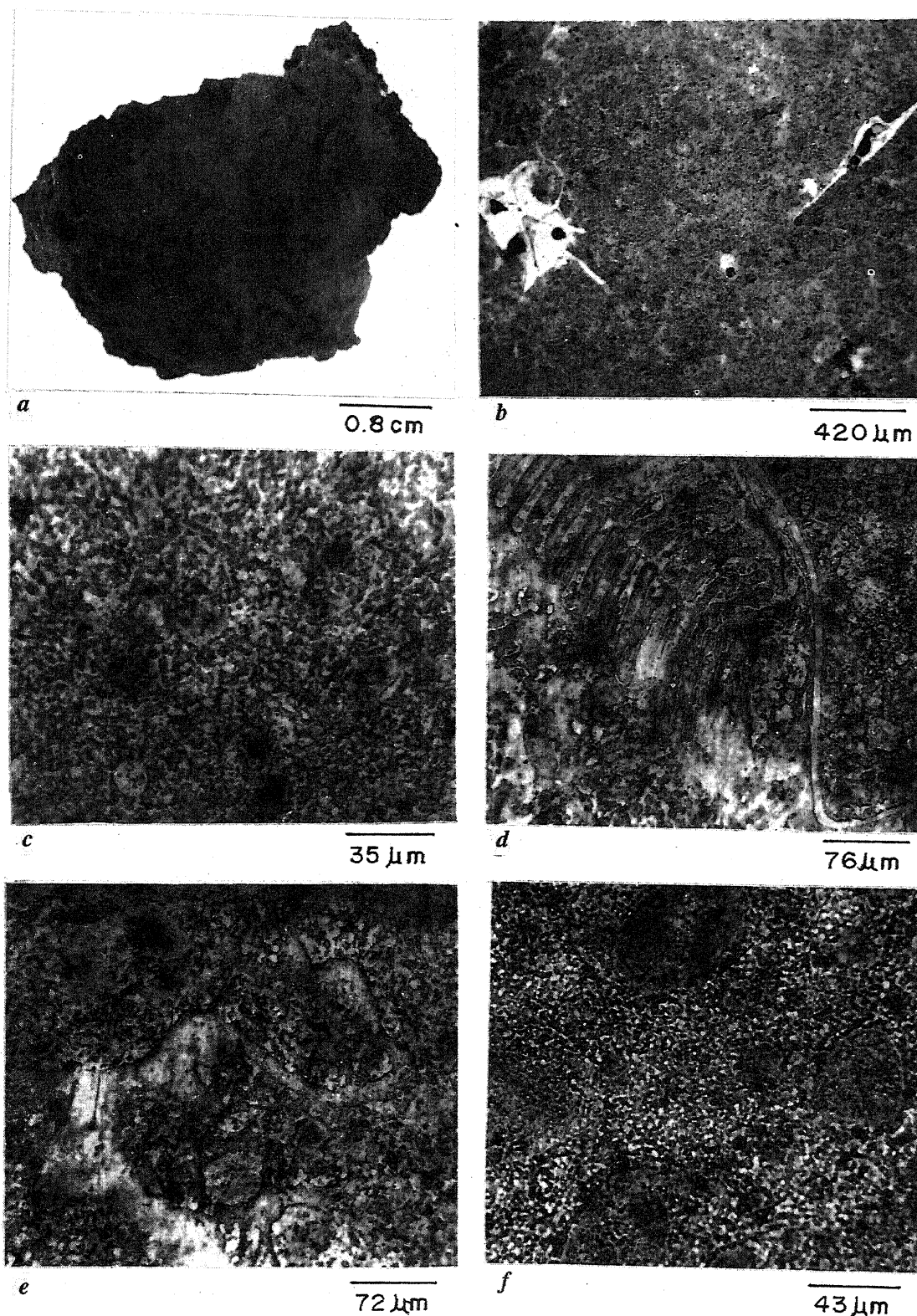
Figure 2. a , Phosphorite crust; ( b-f ) are thin section photomicrographs; b , at low magnification showing homogeneous apatite structure with a few bone fragments; c , high magnification showing porous microstructure; d , fish bones being micritized; e , bone fragment showing phosphomicritization; f , the end product of phosphatization of bones showing undifferentiated phosphate peloids.
