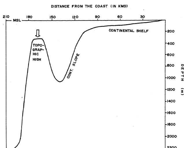
Figure 1. Schematic cross section of the continental margin off Goa showing topographic high on the continental slope; arrow shows the core location (data provided by Dr M. Veerayya).
