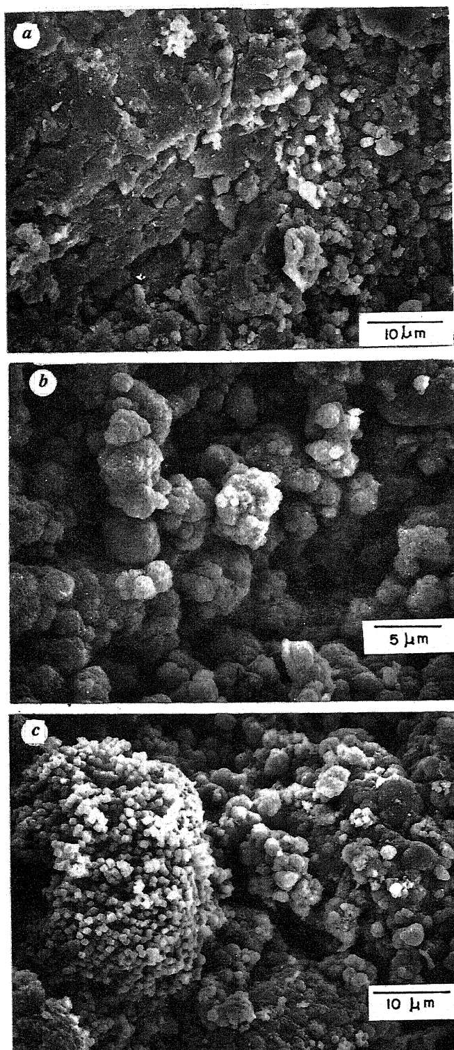
Figure 4. a-c , SEM photographs. a , apatite microstructure with moderately compact area with adjacent porous areas. b , porous area showing agglomerated apatite globules resembling phosphatized bacteria. c , Pyrite aggregate showing cubes and octoids of pyrite with adjacent area showing porous apatite microstructure corresponding to globules.
