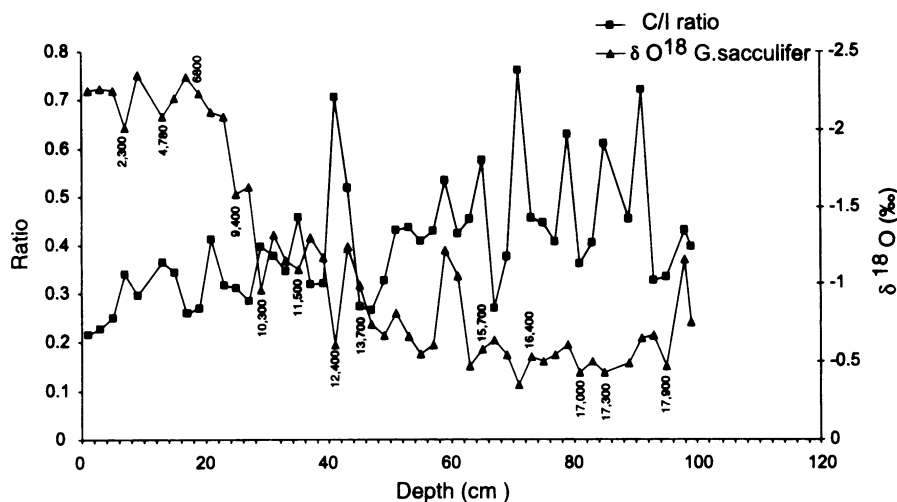
Figure 2. Variations in d^{18}\text{O} in G. sacculifer in the core against aridity indicator C/I ratio. Note a good correlation between heavier incursion of d^{18}\text{O} and higher C/I ratio. Corrected 14 C ages of the levels are shown.
