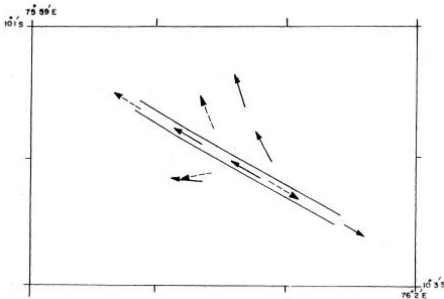
Figure 12. Predicted direction of movement after the disturbance by silt (245° to 310°) (—) and clay (230° to 300°) (---).
