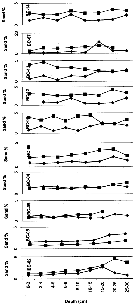
Figure 6. Variation of sand with depth in DZ. ■, pre-disturbance; ◆, post-disturbance.
