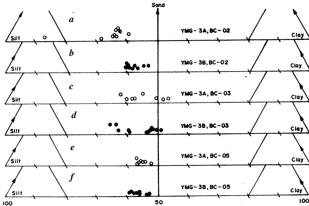
Figure 2. Distribution of sand-silt-clay in DZ ( a, c, e ) before disturbance (open circles, YMG-3 A); and ( b, d, f ) after disturbance (filled circles, YMG-3 B).
