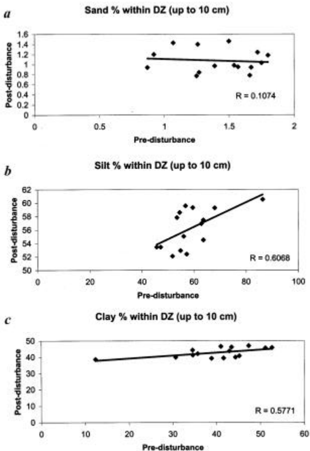
Figure 9. Correlation of pre- and post-disturbed (a) sand %; (b) silt %, and (c) clay %, within DZ.
