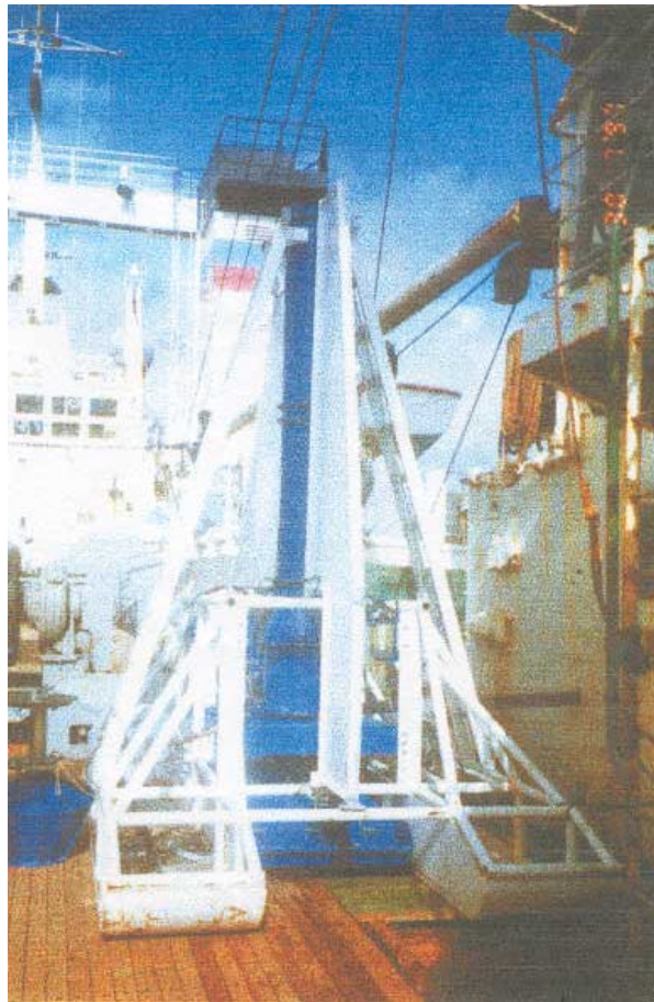
Figure 1. a , Selected sample locations in INDEX area for comparative studies. O, Box core samples before the disturbance; ●, box core samples after the disturbance; \/, INDEX area of disturbance. b , Hydraulic equipment (benthic disturber) used to fluidize and resuspension of the sediments at 5300 m depth in the CIB.
