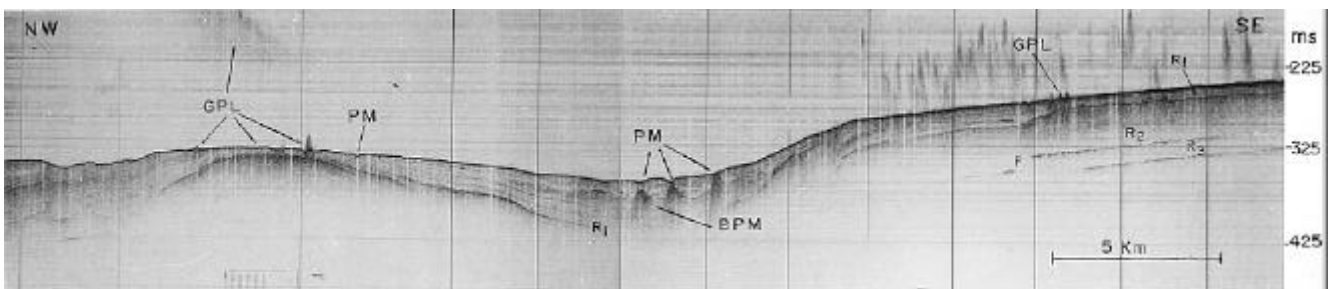
Figure 5. High-resolution ORE sub-bottom seismic profile (3.5 kHz) showing intricate details of gas-related features, such as distinct gas plumes, pockmarks, gas seepages and gas fronts (marked by water column reflections) on the continental slope off Coondapur. Gas plumes (GPL) are seen emanating from the subsurface horizon into the water column. Pockmarks (Pm), buried pockmarks (Bpm), fault (F), prominent reflectors (R1, R2 and R3) are identified in the area. For location see Figure 2.
