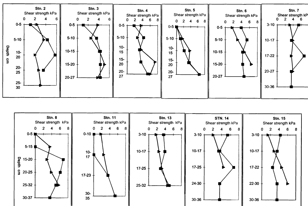
Figure 3. Profiles of shear strength of sediments before (▶) and after (■) the disturbance experiment.
