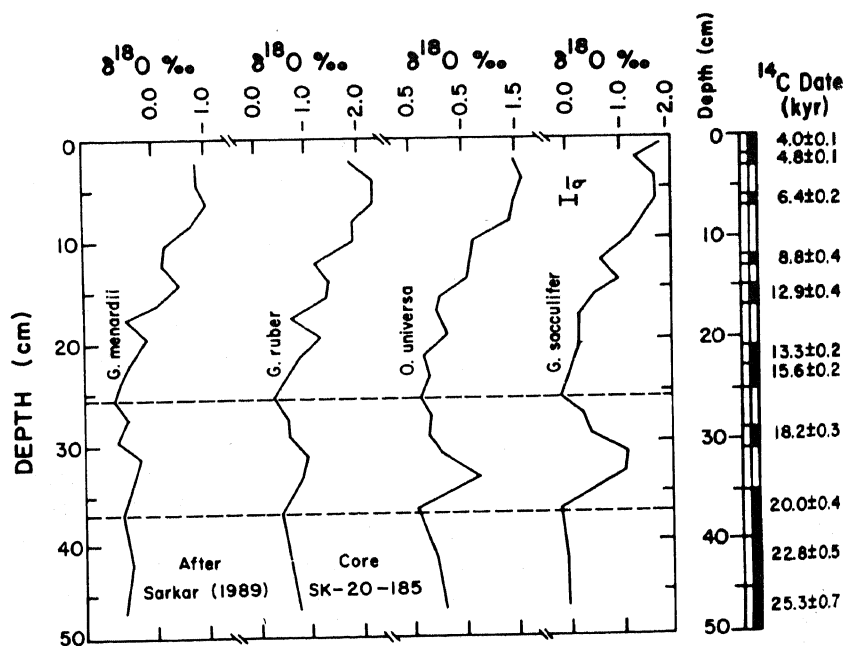
Figure 1. Oxygen isotope data of sediment core SK-20-185 from east Arabian sea, showing the enigmatic negative \delta^{18}\text{O} spike of up to 1‰. This figure replaces figure 1 of ref. 2 in respect of radiocarbon dates.
