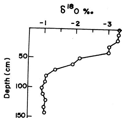
Figure 1. Downcore changes in \delta^{18}\text{O} (‰ versus PDB) in G. ruber in the core MD 77181 ( 17^{\circ}24' \text{ N } 90^{\circ}29' \text{ E} ; water depth 2,271 m (modified from ref. 10).
