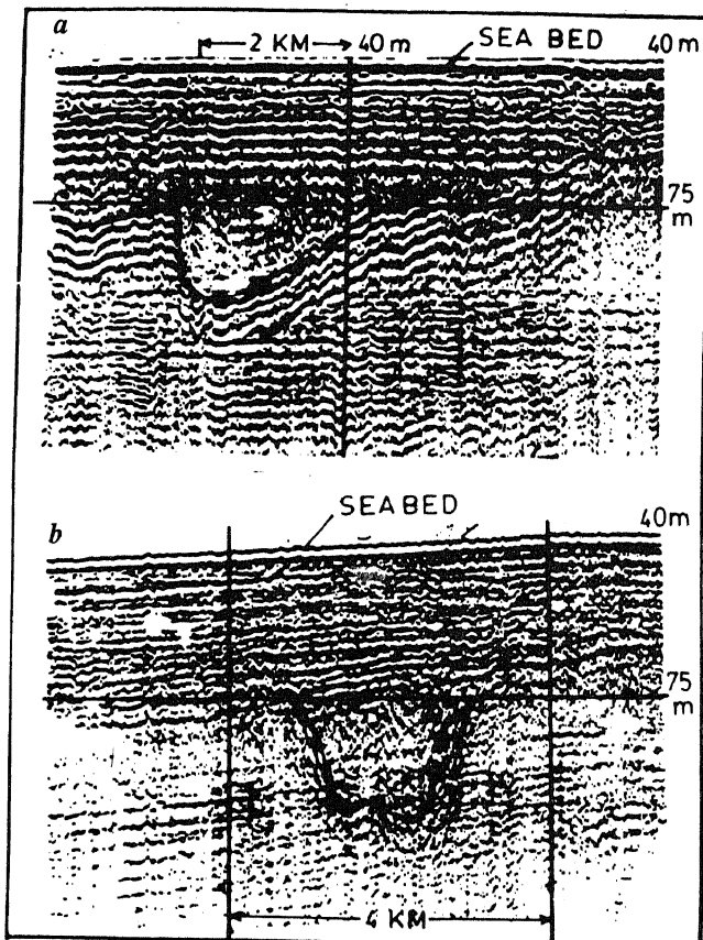
Figure 1 a and b . Buried river channels. a , Off Bhimuniapatnam. b , Off Pudimadaka near Visakhapatnam.
