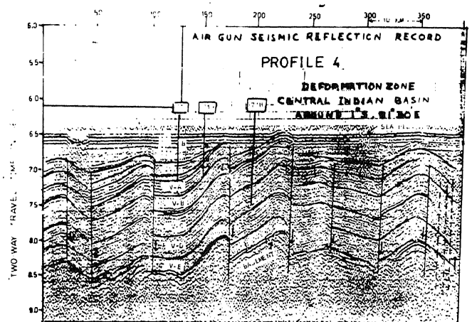
Figure 5. Seismic record over a deformed oceanic crust in Central Indian Ocean Basin.
