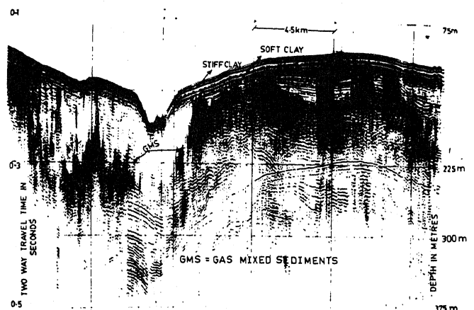
Figure 2. Gas mixed sediments (GMS) off Godavari Basin.
