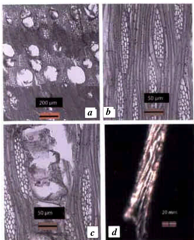
Figure 5. Anatomical analysis of timber of wooden stock from Aguada Bay. Tectona grandis . a, CS showing ring porosity, parenchyma distribution. b, c, TLS showing ray morphology, intervessel pits and septate fibres d. Fibre in polarized light showing soft-rot cavities due to fungal attack.
