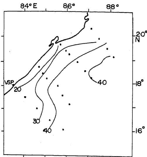
Figure 8. Topography of thickness (m) of surface isothermal layer.
