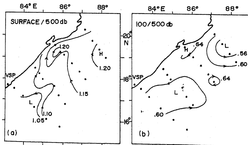
Figure 6. Dynamic topography (dyn. m.) relative to 500 db level surface (a) 0/500 db and (b) 100/500 db.
