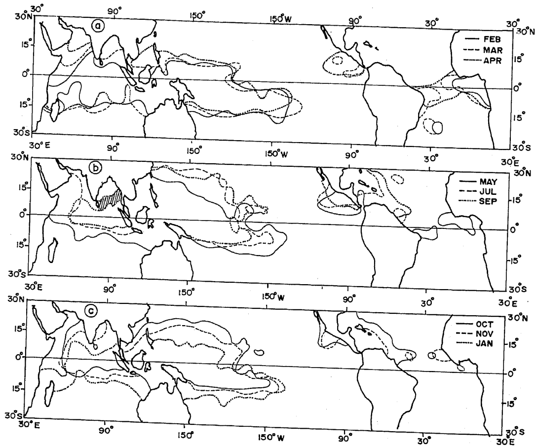
Figure 3. Annual evolution of the tropical warm pool. The contours show 28°C isotherm during (a) February (—), March (---) and April (....); (b) May (—), July (---) and September (....); (c) October (—), November (---) and January (....). During September the warm pool in the Bay of Bengal is split into two parts separated by the shaded portion which is cooler.
