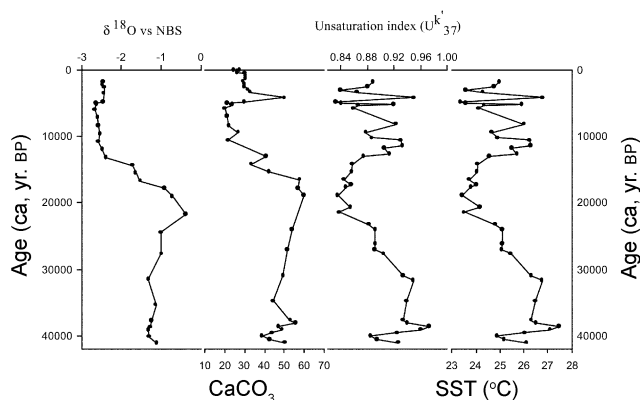
Figure 2. Downcore profiles of d^{18}\text{O} , \text{CaCO}_3 , U_{37}^k and SSTs.
