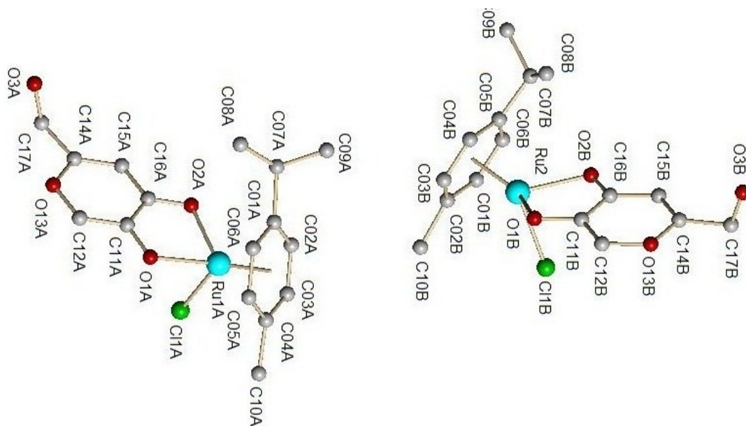
Figure 1. Molecular structure of complex 1 showing two independent molecule A and molecule B. All hydrogen atoms have been omitted for clarity.
