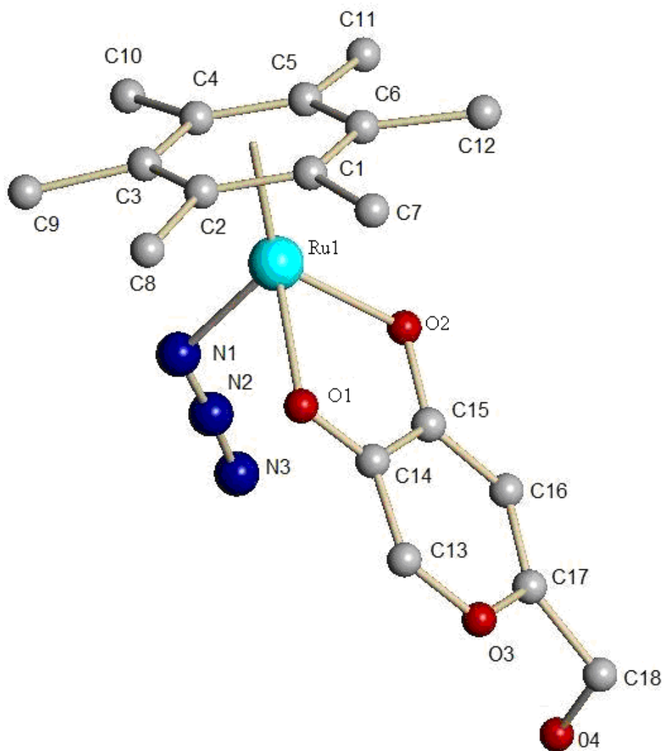
Figure 3: Molecular structure of complex 8 . All hydrogen atoms have been omitted for clarity.
