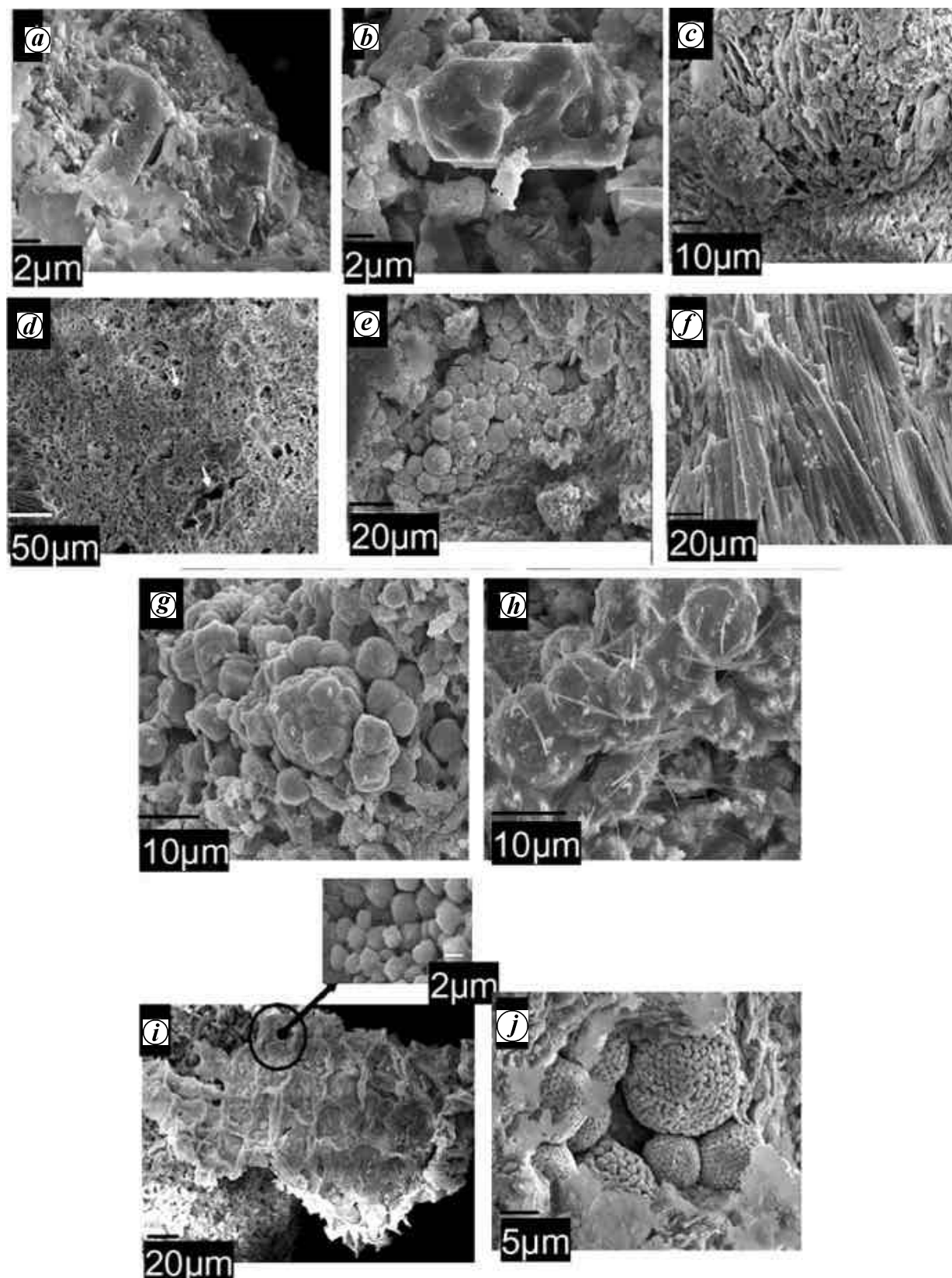
Figure 3. Scanning electron photomicrographs. a , Anhedrals crystals high magnesian calcite (GC-07); b , Euhedral crystals of high magnesian calcite (GC-07); c , Flaky high magnesian calcite with disseminated botryoids (GC-10); d , Porous fabric owing to gas effusion in figure 3 d (GC-13); e , Botryoidal aragonite precipitation within the pore spaces formed by gas effusion in figure 3 d (GC-13); f , Dense fabric of acicular aragonite crystals (GC-13); g , Botryoidal aragonite (GC-13); h , Growth of tender aragonite crystals on the botryoides; i , Remnant of biofilm-like feature with tiny rhomb shaped carbonate crystals (GC-13); j , framboidal pyrite within carbonates and clay matrix from anaerobic sediments (GC-10).
