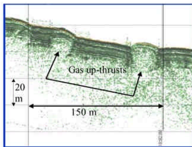
Figure 2. A typical gas up-thrust (gas escape features)-like structure near one of the core locations.
