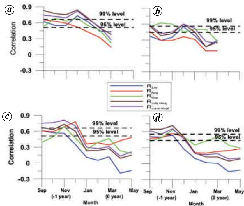
Figure 1. Monthly variation of correlations between SST indices (AS – top; CEIO – bottom) and rainfall for the periods 1978–93 (a, c) and 1978–98 (b, d).
