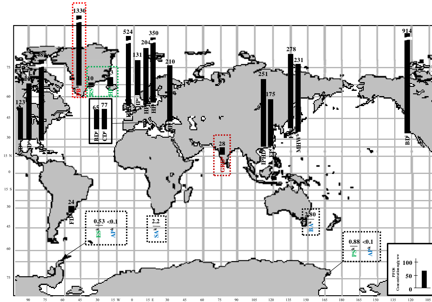
Figure 4. Global comparison of PFOS concentrations in liver samples from different species (marine mammals and seabirds).
