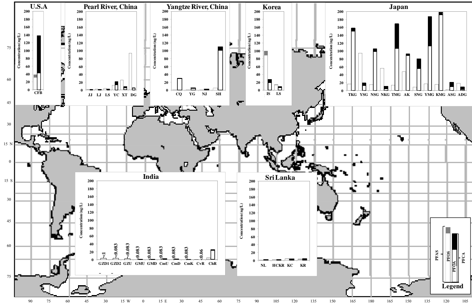
Figure 2. Global comparison of PFOS (PFAS) and PFOA (PFCA) concentrations (ng/L) in river waters.
