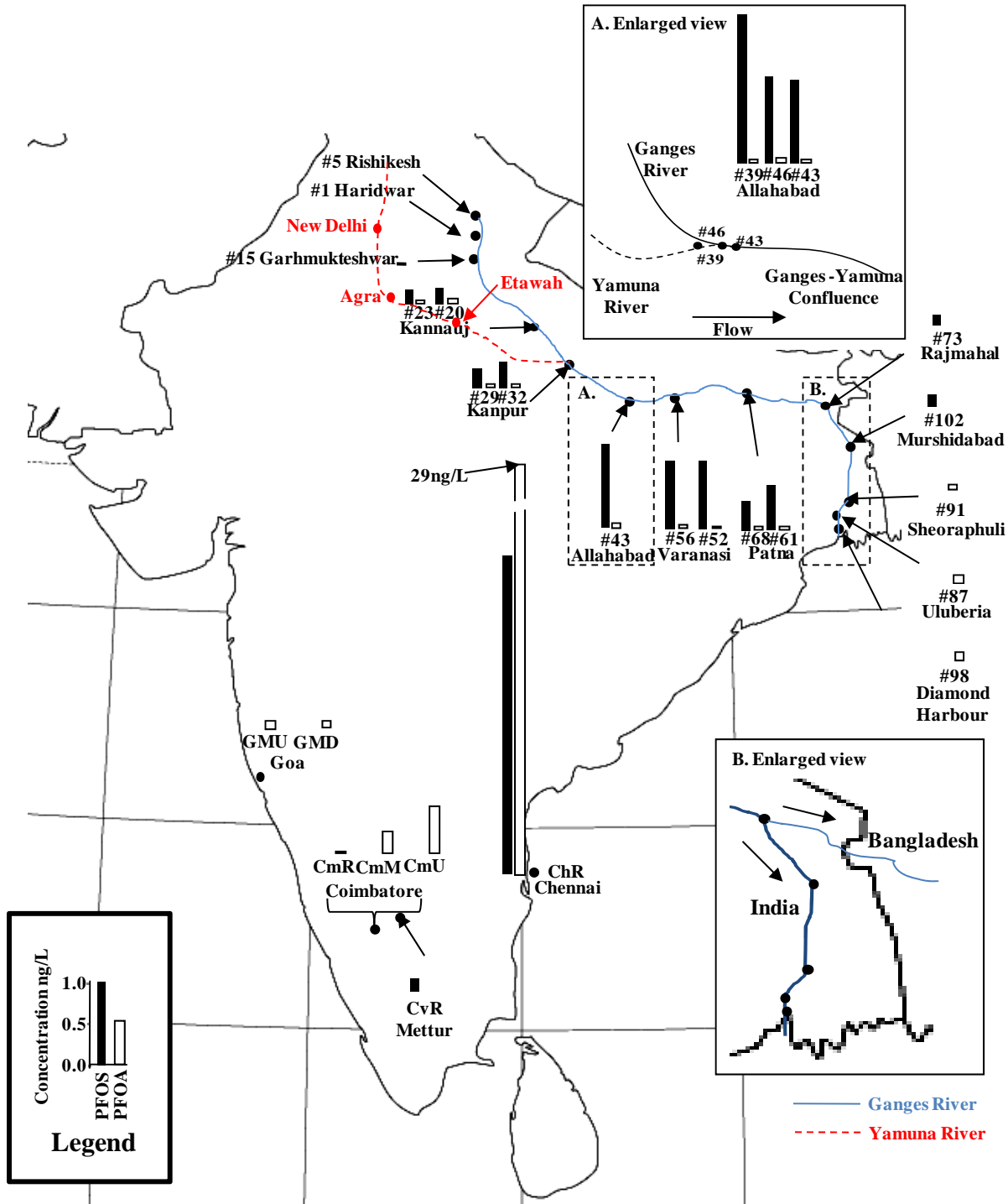
Figure 1 Distribution of PFOS and PFOA in river water samples (ng/L) from India
