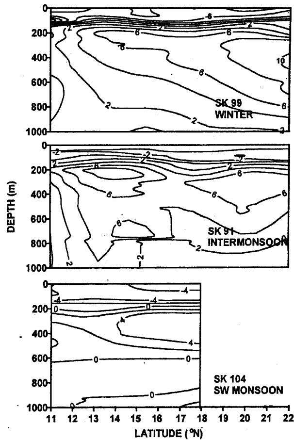
Figure 5. North-south variations in nitrate deficit (DELN, \mu\text{M} ), along 64^\circ\text{E} .
