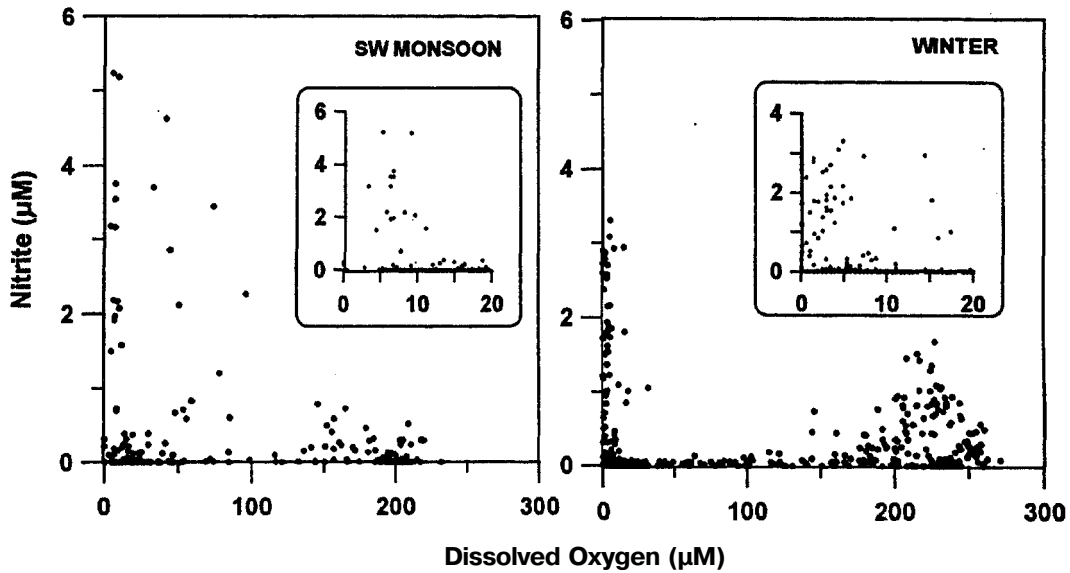
Figure 4. Relation between dissolved oxygen ( \mu\text{M} ) and nitrite ( \mu\text{M} ) during monsoon and winter.
