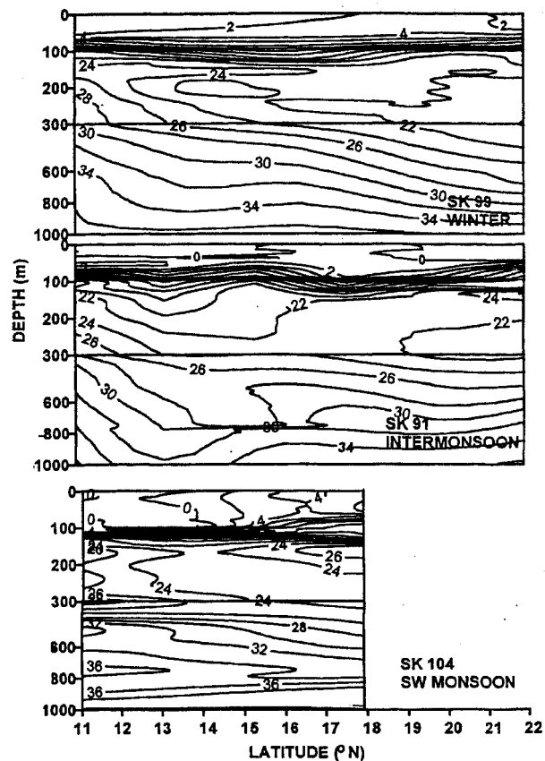
Figure 3. North-south variations in nitrate \mu\text{M} along 64^\circ\text{E} .
