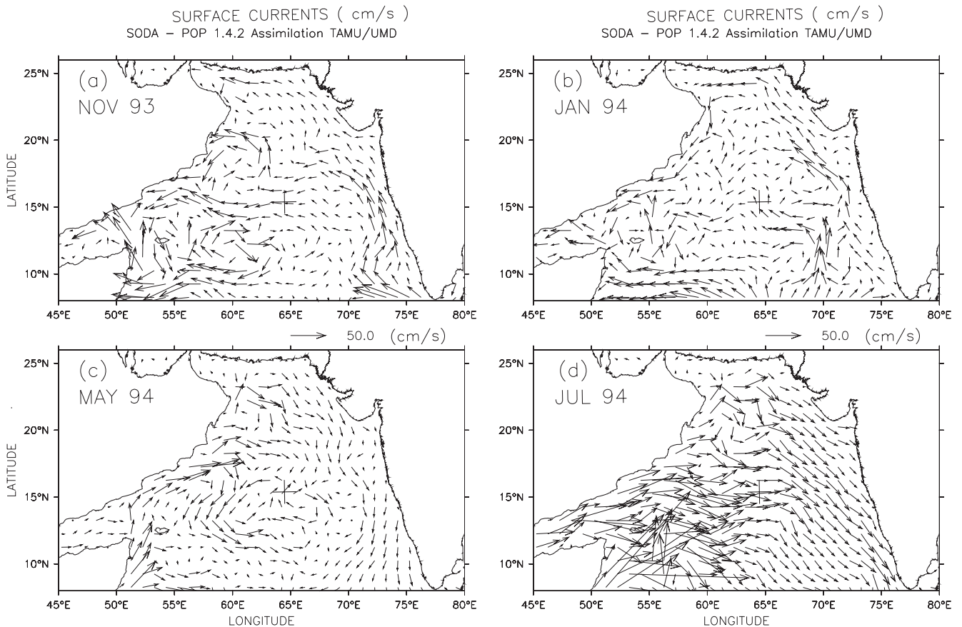
Figure 4. Variation of monthly mean simulated surface currents from Simple Ocean Data Assimilation and Parallel Ocean Program (SODA-POP) [ http://www.dsr.s.atmos.umd.edu/DATA/SODA-1.4.2 ] during (a) November 1993, (b) January 1994, (c) May 1994 and (d) July 1994. For clarity alternate grid current vectors are shown. The sediment trap location is depicted by '+
