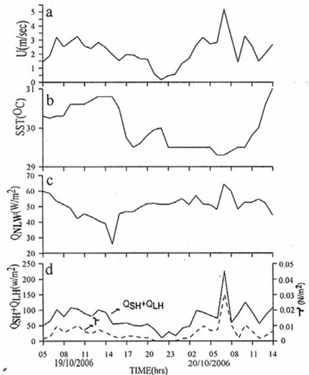
Fig. 2—Diurnal variability of (a) wind speed (m/sec); (b) sea surface temperature ( ^\circ\text{C} ); (c) Net long wave radiation ( Q_{NLW} , \text{W/m}^2 ); (d) enthalpy ( Q_{SH}+Q_{LH} , \text{W/m}^2 ) & wind stress ( \tau , \text{N/m}^2 ) during Phase - I (19 th -20 th Oct. 2006), (Post-monsoon Season)
