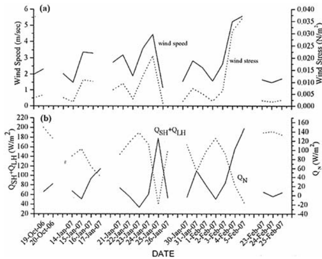
Fig. 7—Daily mean variability of: (a) wind speed (m/sec) and wind stress ( \tau , N/m 2 ); (b) Net heat flux (Q N , W/m 2 ) and enthalpy (Q SH +Q LH , W/m 2 )
