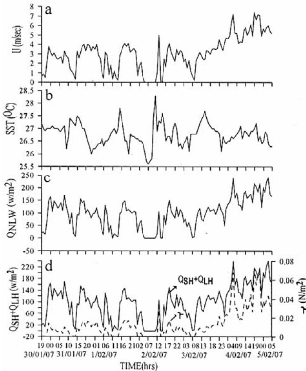
Fig. 5—Same as Fig.4 but during Phase-IV (30/01/07 to 05/02/2007) (Winter Season)
