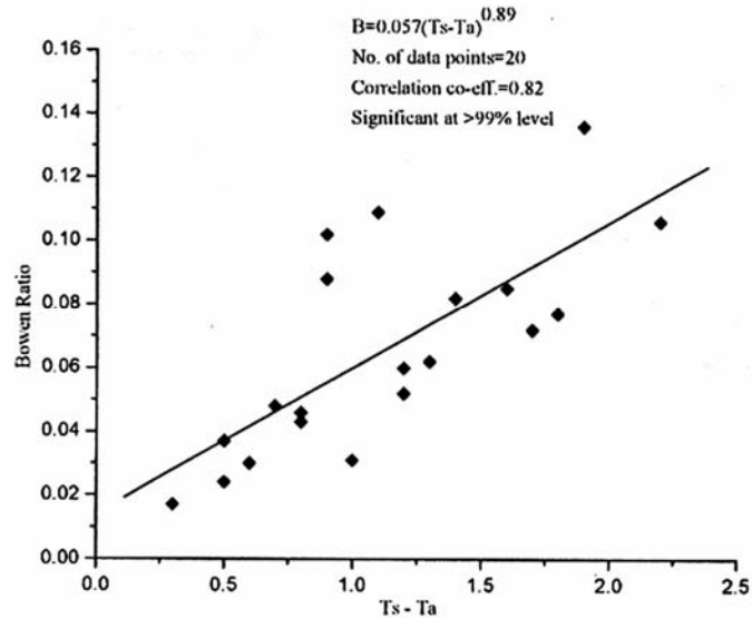
Fig. 8—Scatter plot between Bowen ratio (B) and sea-air temperature difference (Ts-Ta) under unstable conditions
