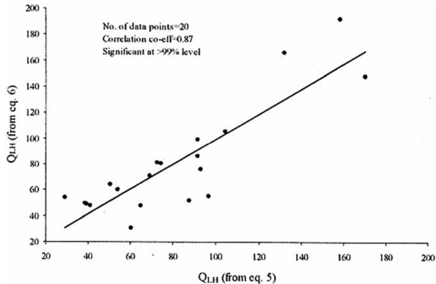
Fig. 9—Scatter plot between the computed (from eq. 5) and estimated values of Q_{LH} from the present method (eq. 6)
