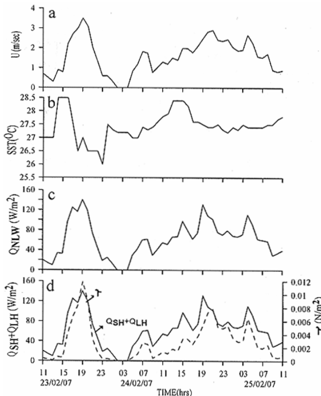
Fig. 6—Same as Fig.5 but during Phase- V (23/02/07 to 25/02/2007) (Winter Season)
