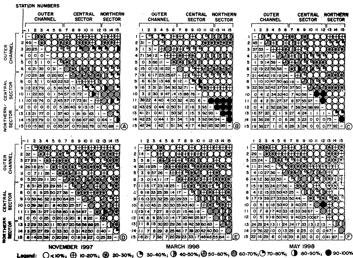
Fig. 3. Trellis diagrams based on Bray-Curtis coefficient (abundance of species), (A,B and C) and Community coefficient (presence or absence of species), (D,E and F) showing percentage affinity index between stations for areas of the lake in different months.
