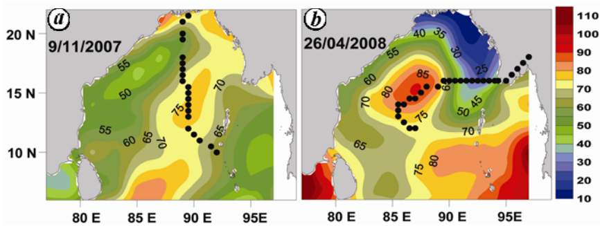
Figure 2. Distribution of UOHC ( \text{kJ}/\text{cm}^2 ) prior to (a) Sidr and (b) Nargis . Storm tracks (dotted line) are also shown.
