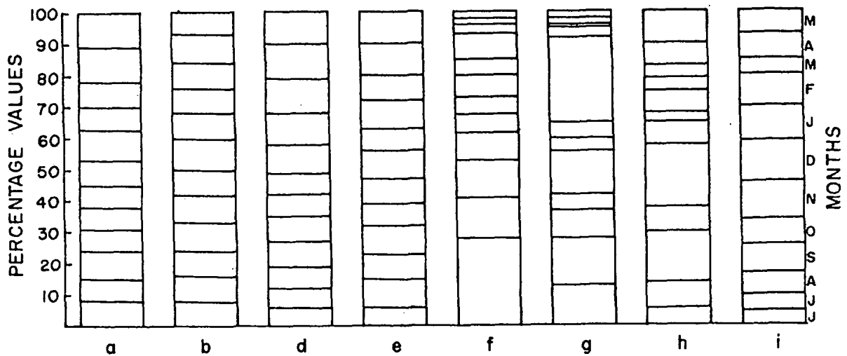
Fig. 8. Percentage distribution of heterotrophic bacteria (a), temperature (b), organic carbon (c), salinity (d), dissolved oxygen (e), PO_4 -P (f), NO_2 -N (g), NO_3 -N (h) and Ammonia (i) in the water table level during high tide.
