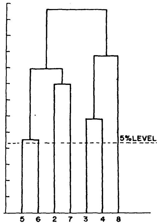
Fig. 12. Dendrogram showing the relationship between water quality parameters, temperature (2), salinity (3), dissolved oxygen (4), PO 4 -P (5), NO 2 -N (6) NO 3 -N (7) and NH 4 -N (8) in the water table level during high tide.
