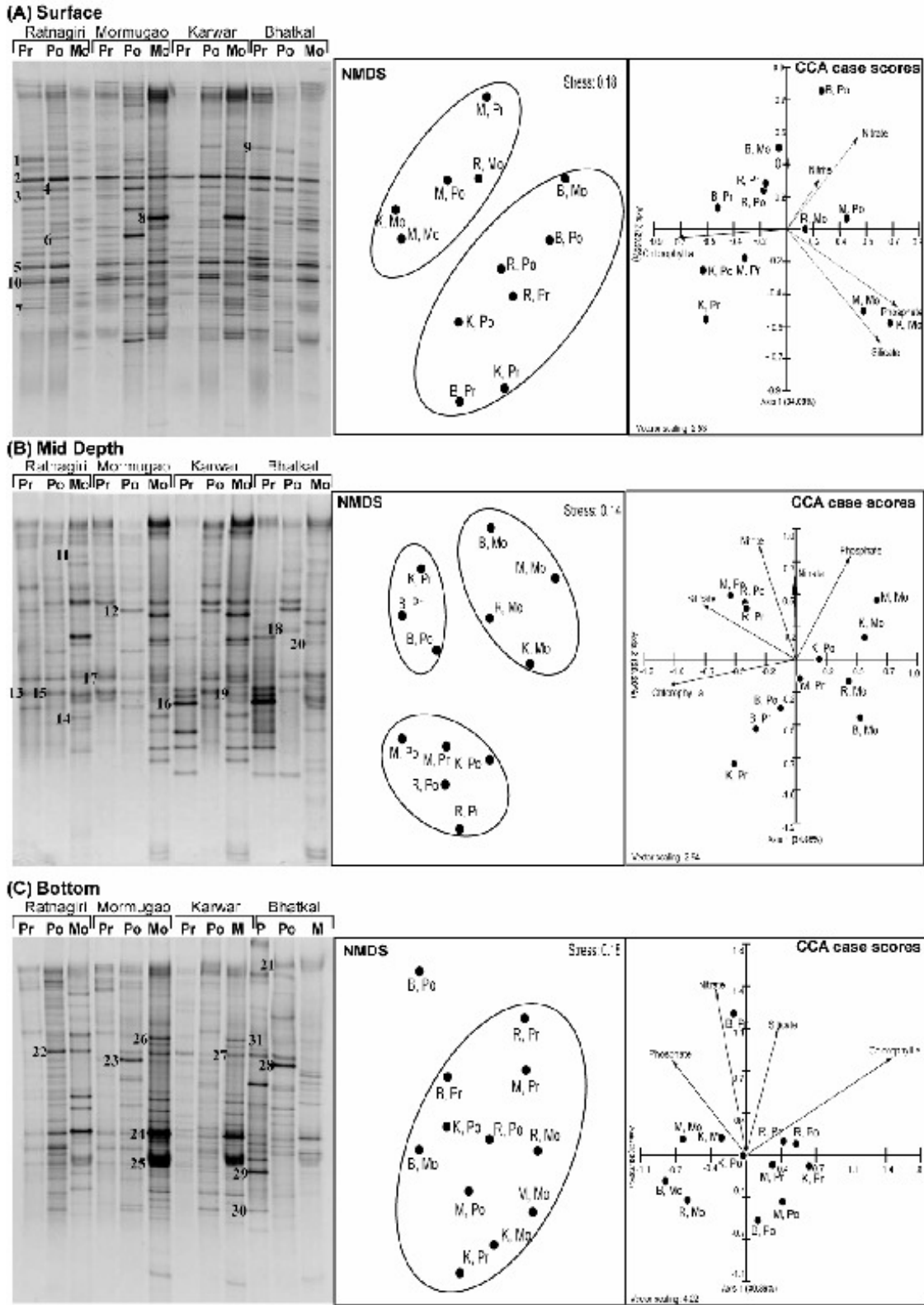
Fig. 3: Spatio and temporal variations in bacterial communities deciphered through DGGE patterns. Samples were collected during premonsoon (Pr), postmonsoon (Po) and monsoon (Mo) off Ratnagiri (R), Mormugao (M), Karwar (K) and Bhatkal (B) from surface (A), mid-depth (10 m; B) and bottom (20 m; C). Results from non-metric dimensional scaling (NMDS) and canonical correspondence analysis (CCA) are also included for each gel. The percentages of variations explained through CCA by each axis are in parentheses. Very small vectors are not shown
