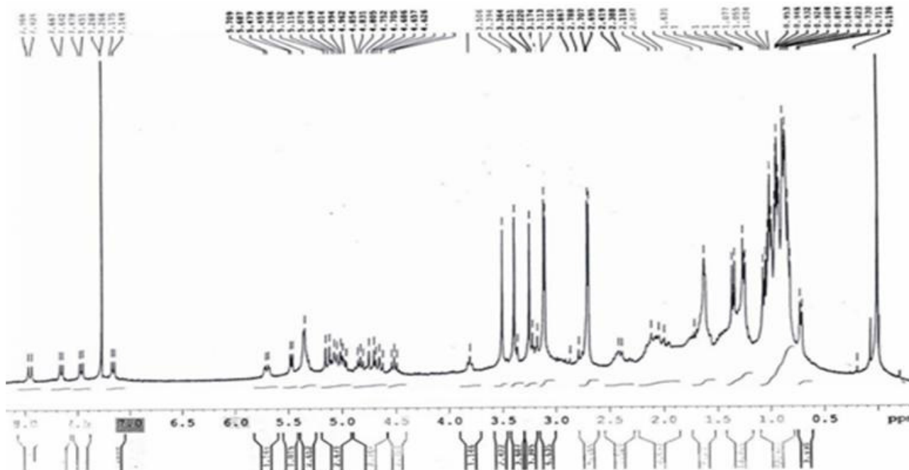
Fig. 2: ^1\text{H} NMR spectrum of purified Cyclosporine A
