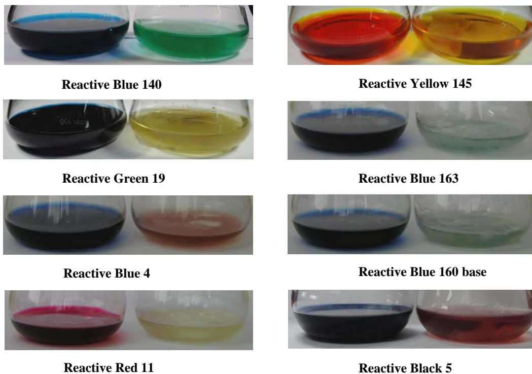
Fig. 2.9: Decolorization of Reactive dyes by representative fungi.
