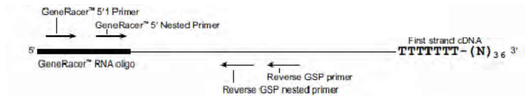
Fig 7.2 The 5'ends of the cDNA are amplified using a reverse gene specific primer and the GeneRacer 5' primer. In this amplification only the mRNA which have GeneRacer RNA oligo attached to its 5' and which is completely transcribed is amplified. (Invitrogen handbook)
