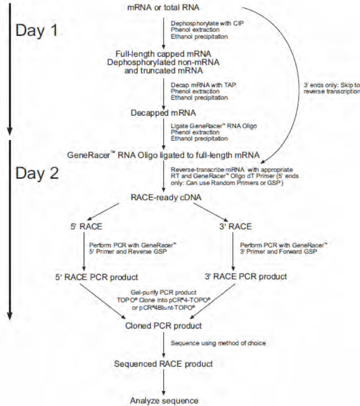
Fig 7.1 Flow chart for the Gene Racer protocol showing the steps involved in generation of the 5' and 3' end cDNA products. The protocol describe a two day long protocol, starting with Day 1 where the mRNA is decapped and RNA oligo is ligated, on the day 2 the mRNA is reverse transcribed into cDNA and 5' and 3 ends are later generated and finally they are sequenced directly or cloned into vector (Invitrogen handbook)
