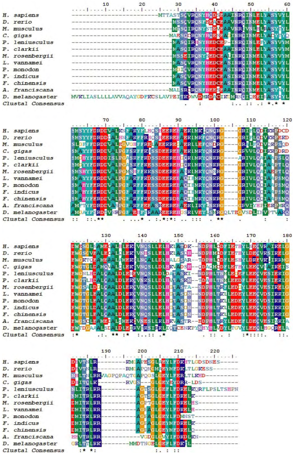
Fig 7.8 Multiple sequence alignment of Ferropenaeus indicus ferritin amino acid sequence obtained in this study (Accession No gb|JN651914|) with other representative ferritin sequences. Identities are marked in asterisk below and similarities are shaded in colored codes.
