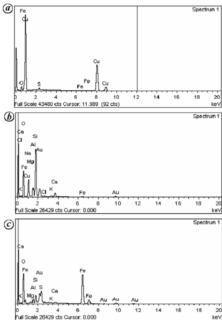
Figure 4. Representative SEM-EDS spectra of copper slag (a), glass ingot (b) and iron concretion (c).
