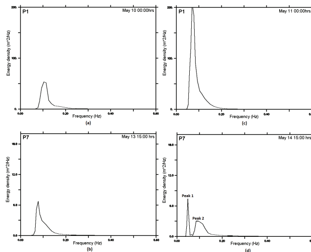
Fig. 8. Typical 2-D energy spectra at two locations P1 and P7 (a) and (b) before and (c) and (d) during the event in May 2007.
