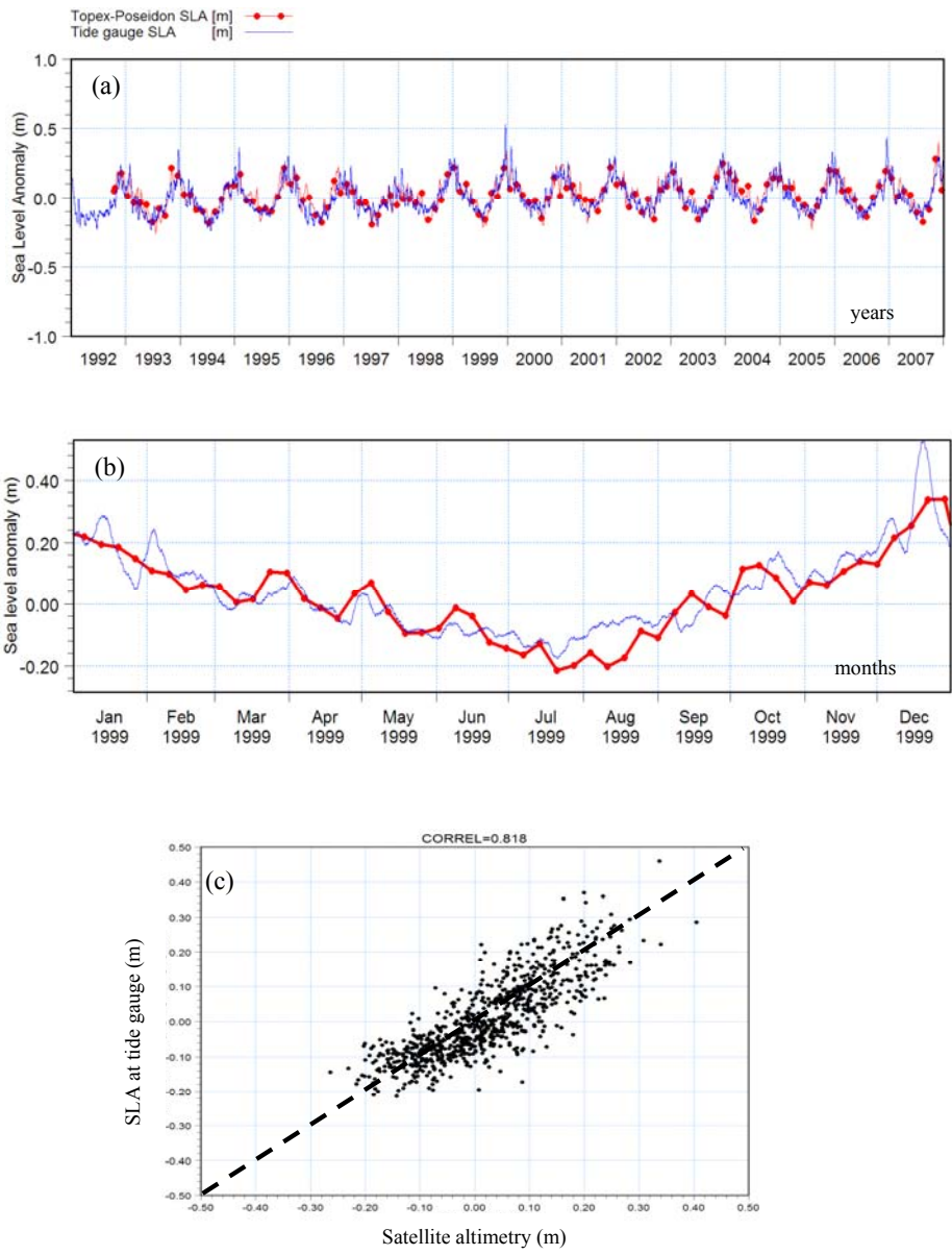
Fig. 2 Sea level anomalies: (a,b) derived from Tanjong Pagar tide gauge and satellite altimetry; (c) correlation between tide gauge and satellite altimetry data.
