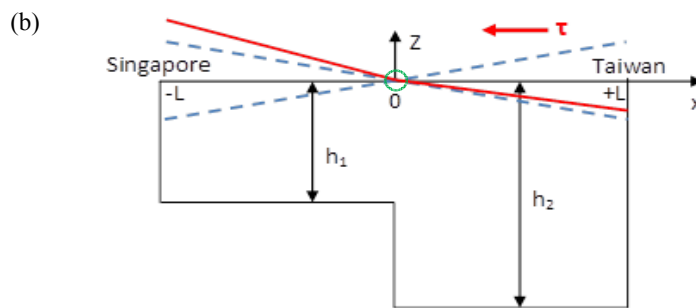
Fig. 11 Conceptual model of storm surges in a channel: (a) 2-D case, (b) 1-D model of the steady state set-up (solid red line) and free oscillations (dashes grey lines) along the main axis of the SCS shown in Fig 5 during the northeast monsoon. Nodal point over shelf break is shown by a circle.
