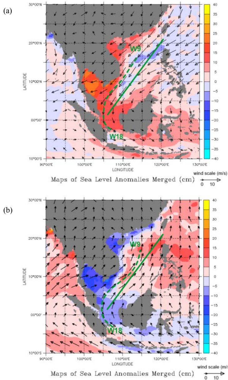
Fig. 3 Climatological seasonal 6-hourly wind and satellite altimetry averaged over 1993 - 2008 years: (a) NE Monsoon (Nov, Dec and Jan Feb), (b) SW Monsoon (Jun, Jul and Aug). Solid line is the longest axis of Taiwan-Singapore and dash-lines are the wind speed streamlines.
