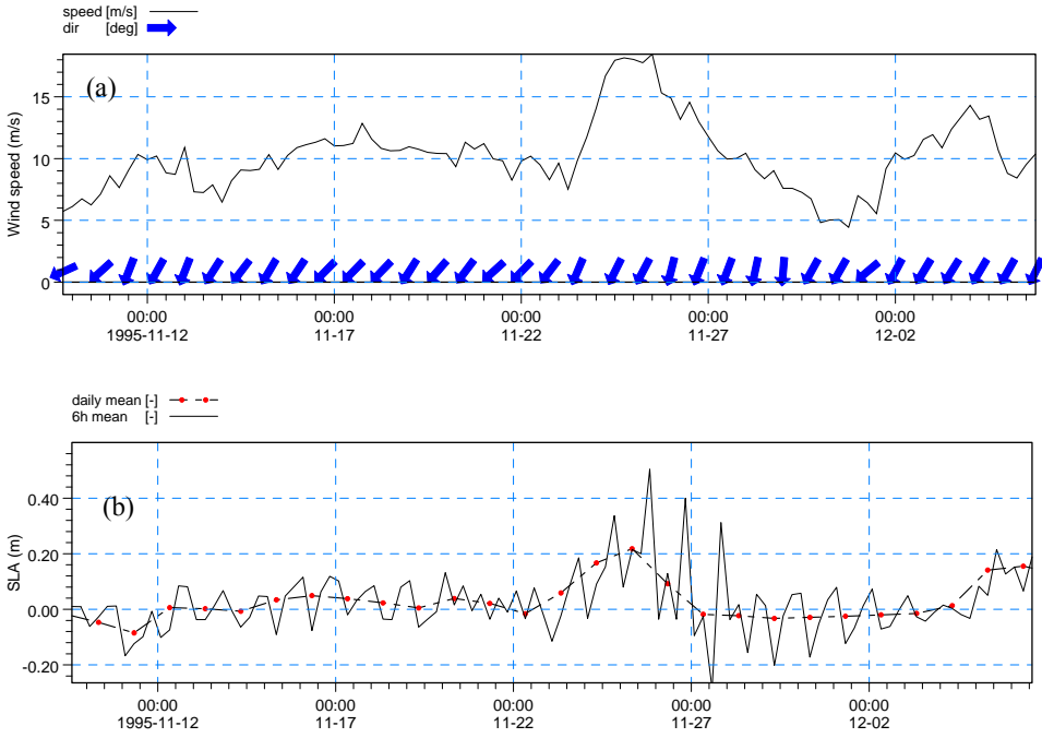
Fig. 9 (a) NCEP wind speed and direction at 12.5°N and 112.5°E, (b) sea level anomaly at Tanjong Pagar during the highest spring tide of 25 November 1995
