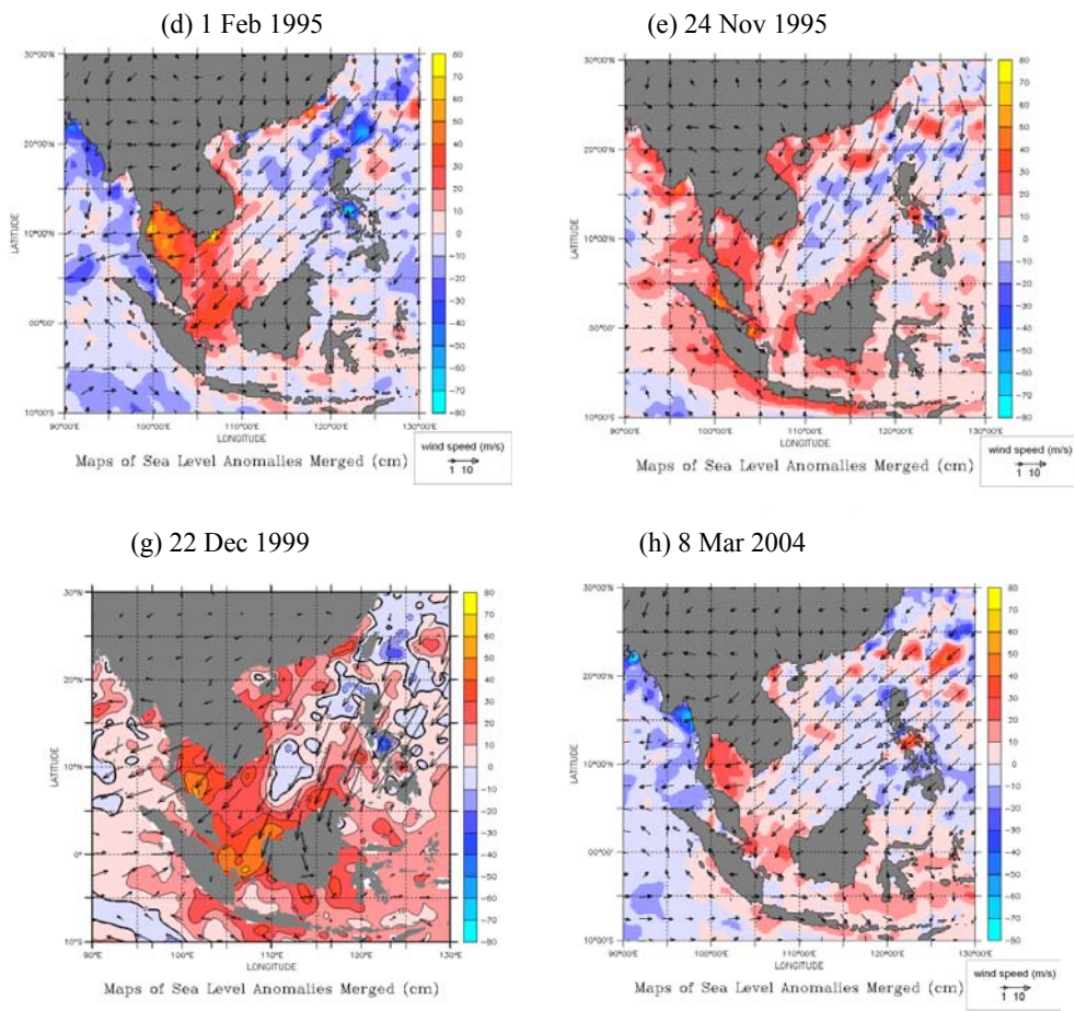
Fig. 8 Selected extremes of sea level anomalies overlapped with corresponding wind.
