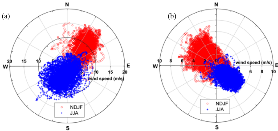
Fig. 4 Climatological wind rose diagrams for the period 1984 – 2007 at wind cells (Fig. 1a): (a) wind cell W9 (off Vietnam), (b) wind cell W18 (Karimata Strait). NE monsoon wind is depicted by red circles, while SW monsoon wind is shown by blue crosses.
