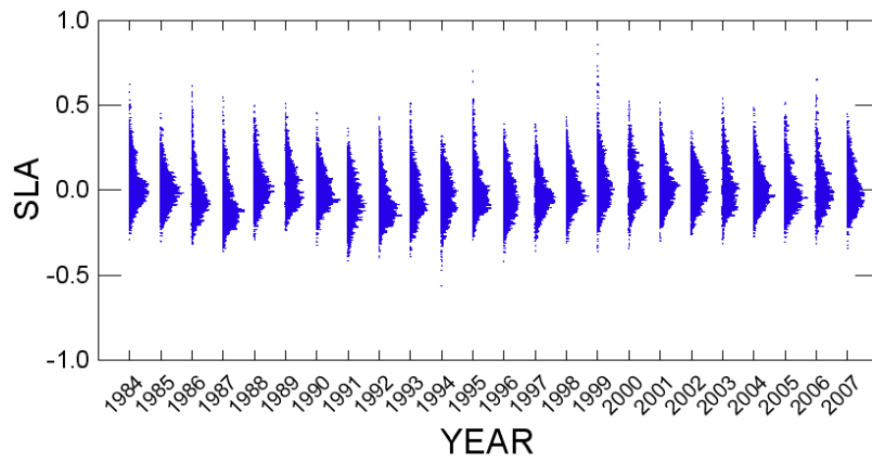
Fig. 7 Annual frequency distribution of SLAs
