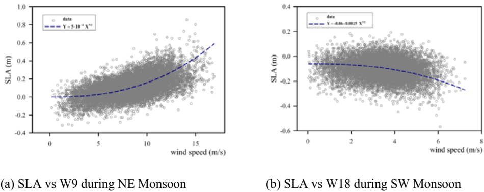
Fig. 12 Dependence of SLA in Singapore Strait on wind at selected 5° cells (as in Fig. 1a)
