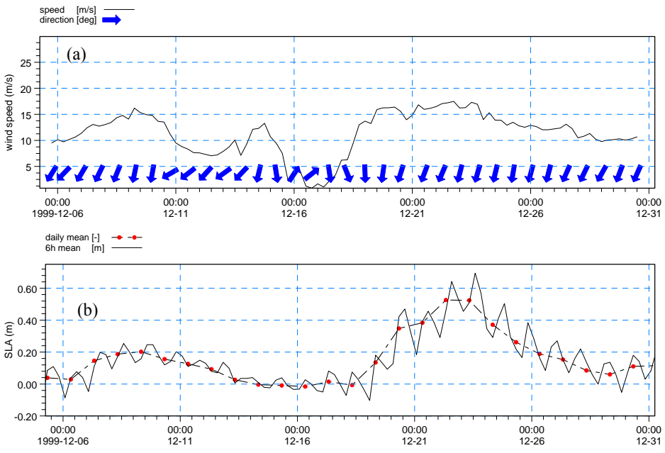
Fig. 10 (a) NCEP wind speed and direction at 15°N and 110°E, (b) extreme sea level anomaly (without annual and semi-annual components) at Tanjong Pagar during the highest spring tide of 23 December 1999
