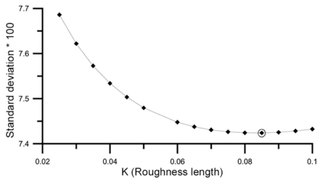
Figure 3. Calibration of bottom roughness length ( k ) with standard deviation.
