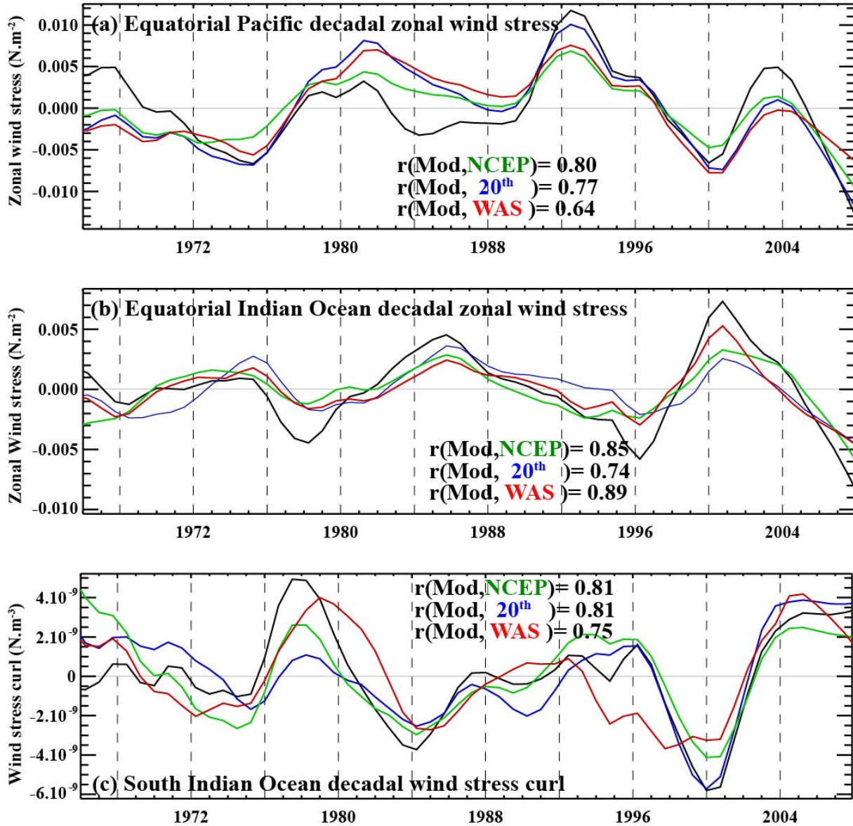
Figure 9: Time series of decadal (a) equatorial Pacific zonal wind stress ( 140^{\circ}\text{E}-140^{\circ}\text{W} ; 2.5^{\circ}\text{N}-2.5^{\circ}\text{S} ; red box on Fig. 8a), (b) equatorial Indian Ocean zonal wind stress ( 60^{\circ}\text{E}-100^{\circ}\text{E} ; 2.5^{\circ}\text{N}-2.5^{\circ}\text{S} ; green box on Fig. 8b) and (c) south Indian Ocean wind stress curl ( 60^{\circ}\text{E}-110^{\circ}\text{E} ; 20^{\circ}\text{S}-5^{\circ}\text{S} ; yellow box on Fig. 8b) from model output (black line, similar to ERA40), NCEP reanalysis (green line), 20 th century reanalysis (blue line) and WASWind dataset (red line). Units are in \text{N.m}^{-2} for wind stress and \text{N.m}^{-3} for wind stress curl. The correlation between the model forcing and other datasets is indicated on each panel.
