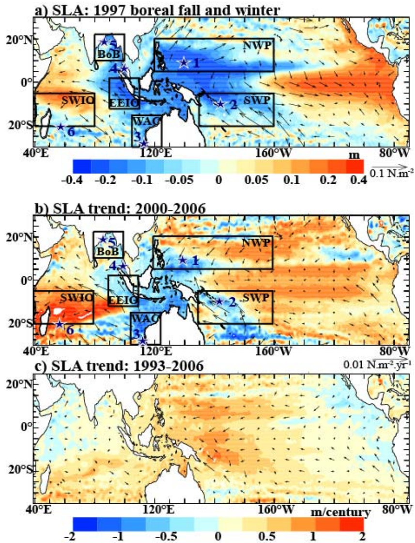
Figure 1: (a) Satellite SLA during October 1997-March 1998 (color) and associated wind anomaly derived from NCEP (arrow). (b) Satellite SLA linear trend for the 2000-2006 period (color) and associated NCEP wind stress trend (arrow). (c) Satellite SLA linear trend for the 1993-2006 period (color) and associated NCEP wind stress trend (arrow). The mean seasonal cycles were removed from both SLA and wind datasets. The stars on panels (a) and (b) indicate locations of the tide-gauges used to validate the model sea level. The selected gauge locations are (1) Yap B (138E ; 9.5N), (2) Honiara II (161E ; 9.5S), (3) Fremantle (115.7E ; 32S), (4) Langkawi (99.8E, 6.4N), (5) Paradip (86.7E ; 20.3N) and (6) Port Louis (57.5E ; 20.15S). Boxes on panel (a) and (b) indicate the regions where model will be validated to satellite observations. The selected boxes are the North West Pacific (NWP), the Western Australian Coast (WAC), the South West Pacific (SWP), the Eastern Equatorial Indian Ocean (EEIO), the Bay of Bengal (BoB) and the South West Indian Ocean (SWIO). Panel (b) is identical to figure 1c of Lee and McPhaden (2008), i.e. an estimate of decadal sea level variations over that period. Panel (c) provides an estimate of long-term sea level trends over 1993-2006, the period consistent with the study by Lee and McPhaden (2008). Units are in m for panel (a) and m/century for panels (b-c).
