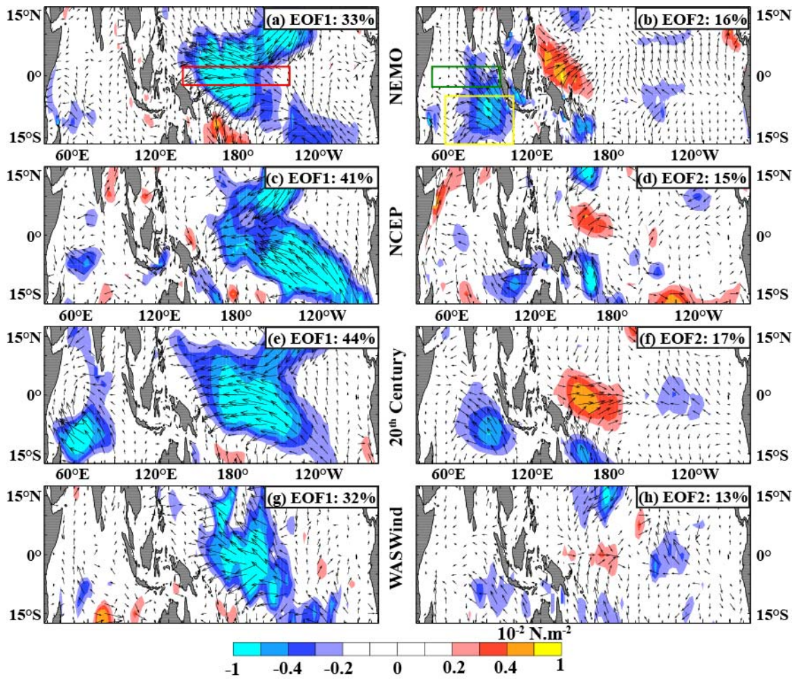
Fig 8: First two EOF patterns of the zonal wind stress over the Indo-Pacific sector at decadal timescale for (a-b) model forcing, (c-d) NCEP reanalysis, (e-f) 20 th century reanalysis and (g-h) WASWind product. The arrows indicate the wind stress components regressed onto the normalized PCs. The percentage variance explained by each EOF is shown in brackets. Units are in \text{N.m}^{-2} .
