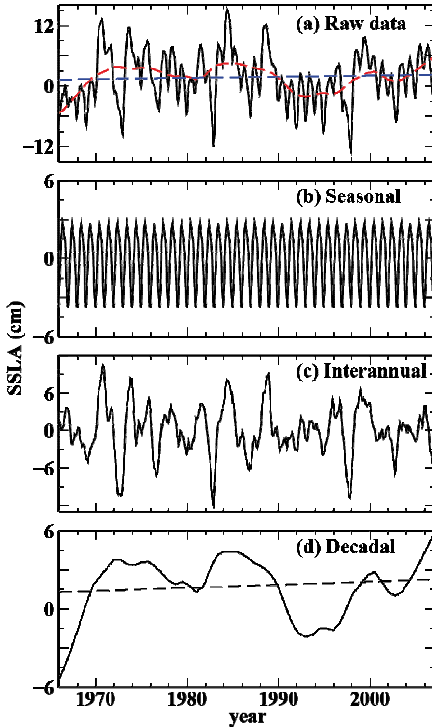
Fig 2: Time series of model steric sea level variations in the Northwest Pacific, extracted by STL method: (a) raw data (black curve), (b) seasonal, (c) interannual and (d) decadal component. The linear trend associated with multi-decadal variability is shown as a dashed line in panel (d). This linear trend has been subtracted from estimates of decadal variability in this paper. The components shown in panel (d) are also shown in panel (a). Units are in m.
