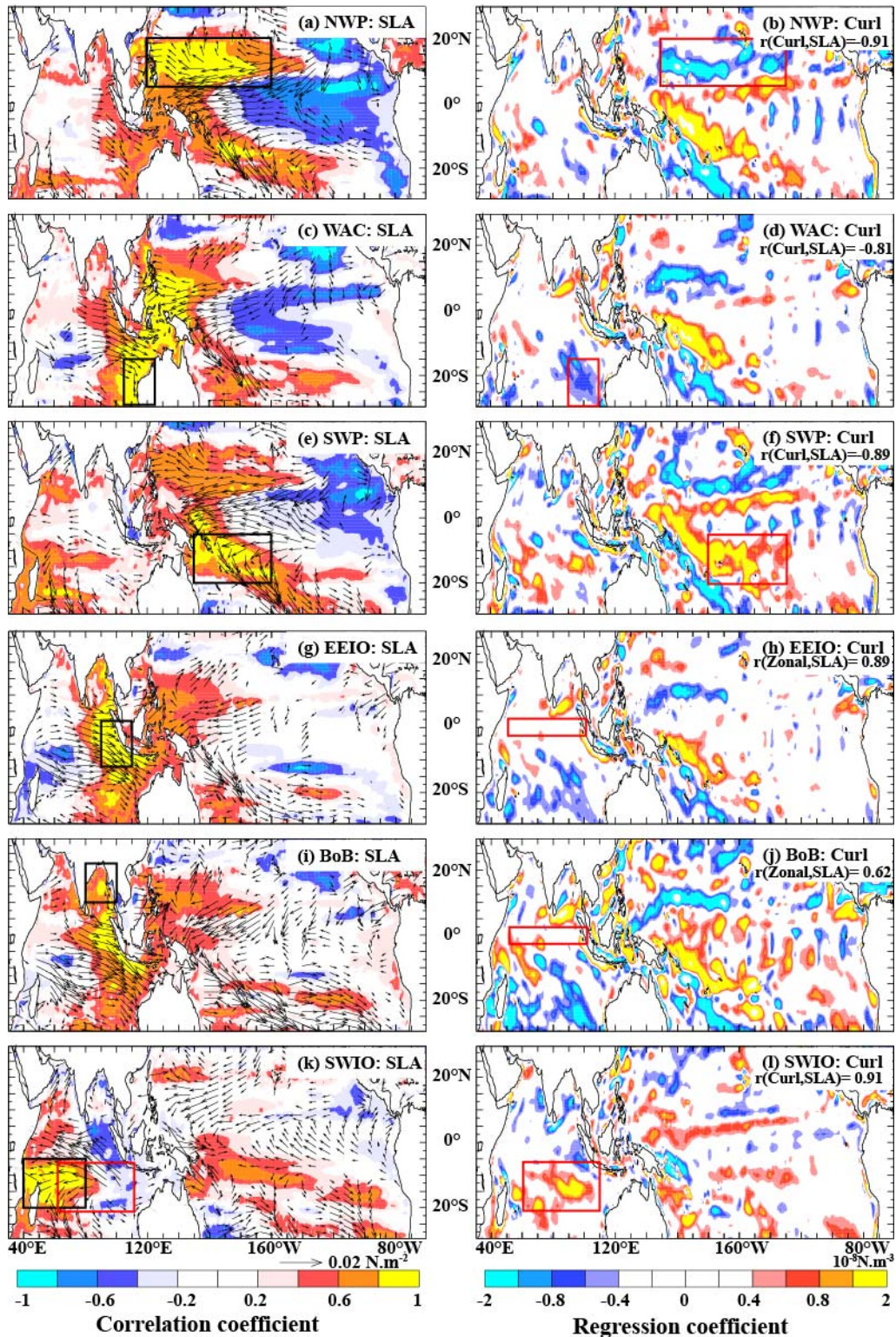
Fig 7: (a) Correlation of model SSLA averaged over the NWP to the entire Indo-Pacific region (color) and regression of wind stress components (arrows) to the model normalized SSLA averaged over NWP. (b) Regression of wind stress curl to the normalized model SSLA averaged over NWP. Same for WAC (c-d), SWP (e-f), EEIO (g-h), BoB (i-j) and SWIO (k-l). The numbers provided below the title in the right column indicate the correlation coefficient between the average SSLA within the black frame (on the left) and average zonal wind stress (or wind stress curl) within the red frame (on the right). Units are in \text{N.m}^{-3} for curl.
