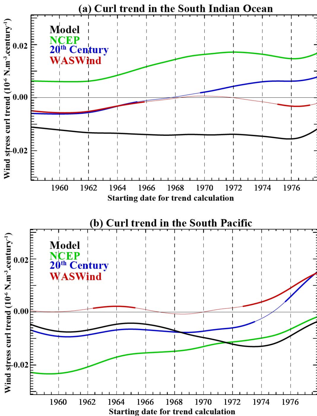
Fig 12: Linear long term trend of the wind stress curl averaged over (a) the south Indian Ocean (60°E-110°E; 20°S-5°S) and (b) the south Pacific (160°E-120°W; 20°S-5°S) for the four wind datasets considered (20 th Century reanalysis, NCEP, WASWind and model), as a function of the starting date of the trend computation period (with this period varying from 1958-2007 to 1978-2007). The bold lines indicate when the trend is significantly different from zero at the 95% confidence level.
