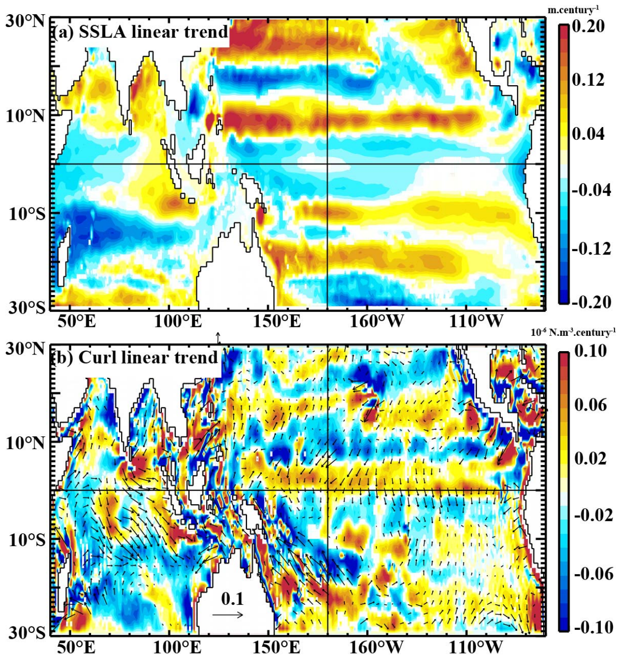
Fig 10: Linear trend over the 1966-2007 period for (a) model steric sea level and (b) model wind stress curl (in colors). The vectors on panel (b) show the wind linear trend. Units are m.century -1 for steric sea level, N.m 3 .century -1 for wind stress curl and N.m 2 .century -1 for wind stress.
