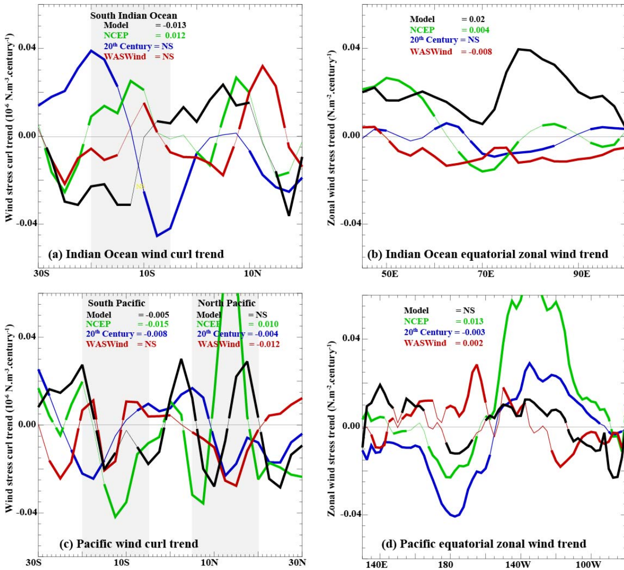
Fig 11: (a) Zonal average wind stress curl linear trend over the Indian Ocean (60°E-110°E) over the 1966-2007 period for the four datasets considered (20 th Century reanalysis, NCEP, WASWind and model). Average wind stress curl linear trend in the South Indian Ocean (20°S-5°S) is also indicated for each dataset. (b) 2.5°N-2.5°S averaged zonal wind stress linear trend over the 1966-2007 period in the Indian Ocean. Average zonal wind stress linear trend in the Equatorial Indian Ocean is also indicated for each dataset. (c) Same as (a) but in the Pacific (160°E-120°W). Average wind stress curl linear trend in the North (5°N-20°N) and South Pacific (20°S-5°S) is also indicated for each dataset. (d) Same as (b) but in the equatorial Pacific. Average zonal wind stress linear trend in the Equatorial Pacific is also indicated for each dataset. Units are \text{N}\cdot\text{m}^{-3}\cdot\text{century}^{-1} for wind stress curl and \text{N}\cdot\text{m}^{-2}\cdot\text{century}^{-1} for wind stress. Bold lines indicate trends that are significantly different from zero at 95% confidence level.
