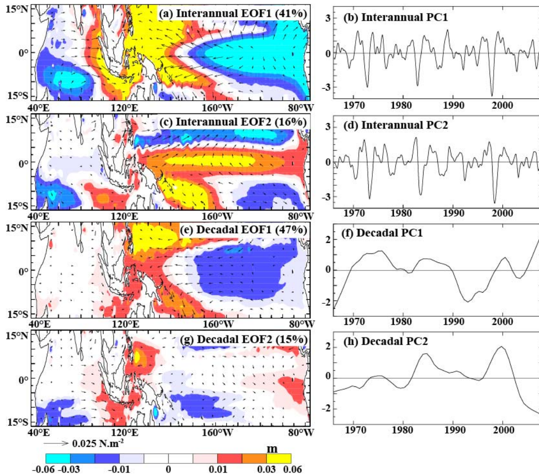
Fig 6: First two EOF patterns of the model steric sea level anomalies over the Indo-Pacific sector (left column) and their corresponding normalized principal components (right column) at interannual ( a-d ) and decadal timescales ( e-h ). The arrows display the wind stress components regressed onto each normalized PCs. The percentage variance explained by each EOF is shown in brackets. Units are in m for EOF patterns and without units for the time series.
