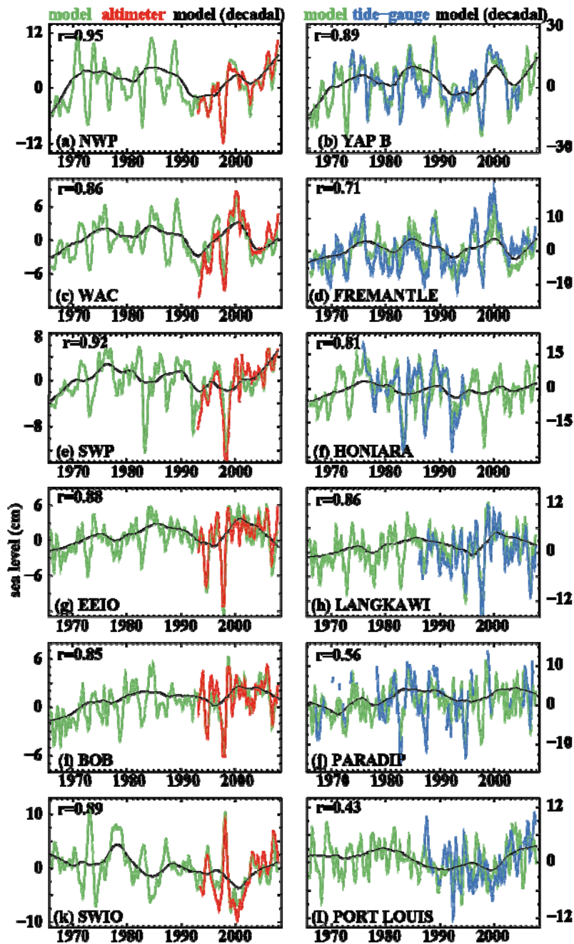
Fig 4: Comparison of monthly model steric sea level anomalies with altimeter (left panel) and tide gauge sea level anomalies (right panel). Time series on the left panels are averaged over the regions shown on Fig 1 and 3 while time series on the right panels are extracted at the corresponding tide gauge locations indicated by stars on Figs 1 and 3. The monthly anomalies were calculated by removing the mean seasonal cycle and a 5 months smoothing was further applied to the time-series. The linear correlation coefficient between the model and observed time-series is given on the top left of each panel. The black line indicates the model decadal signal (including long-term linear trend). Units are in m.
