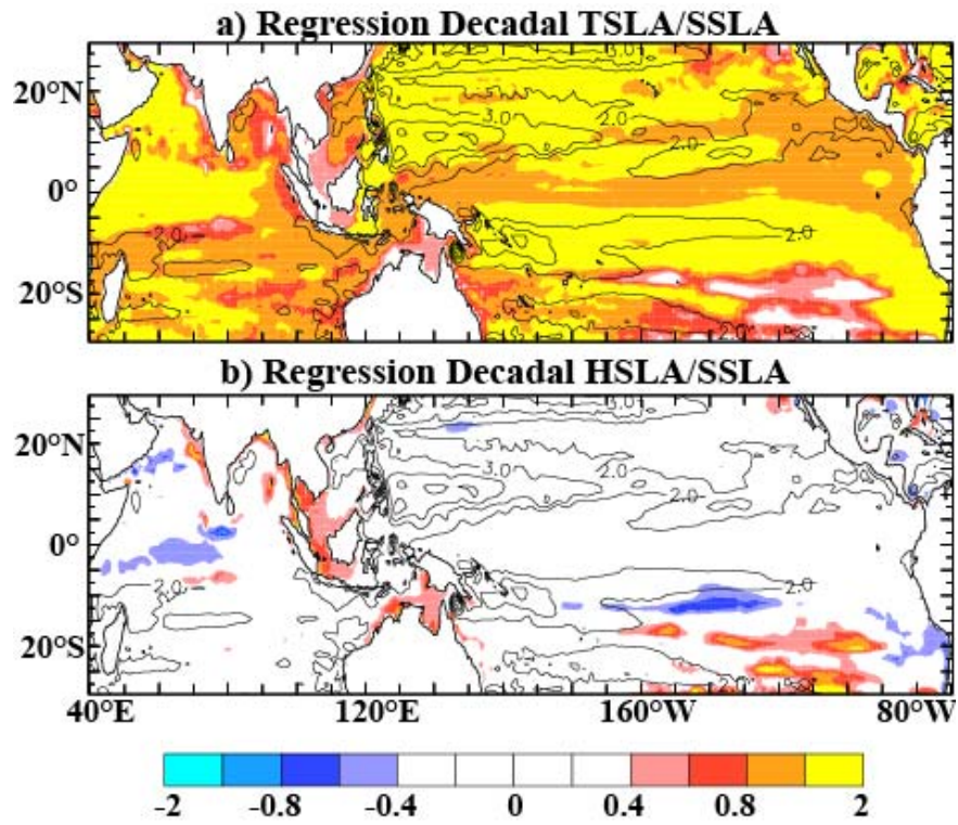
Fig 5: Regression coefficients of model (a) thermosteric and (b) halosteric sea level to model steric sea level at decadal time-scales. The standard deviation of decadal SSLA is also shown by contours on each panel.
