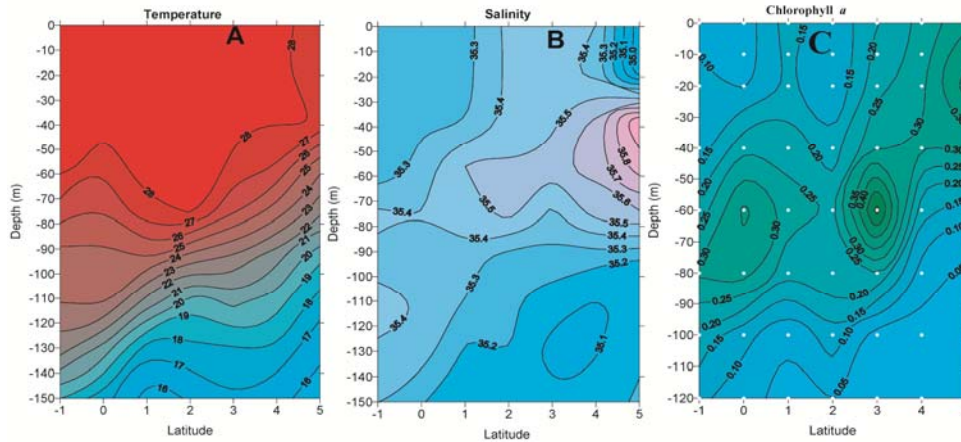
Fig. 2. Vertical profiles of (A) temperature ( ^{\circ}\text{C} ), (B) salinity (psu) and (C) chlorophyll a ( \text{mg}\cdot\text{m}^{-3} ) along 77^{\circ}\text{E} in the EIO during September 2010
